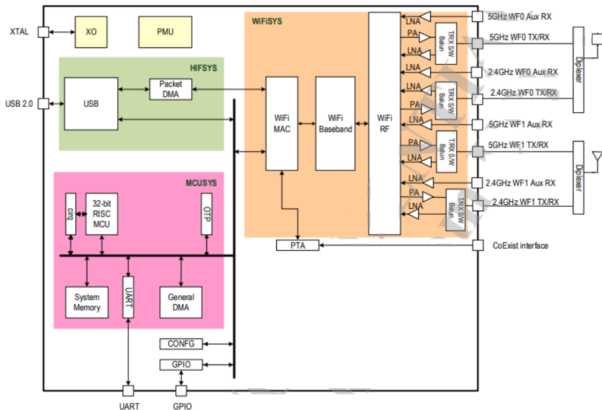
Figure 1 AL-7605B-WG-A Block Diagram
