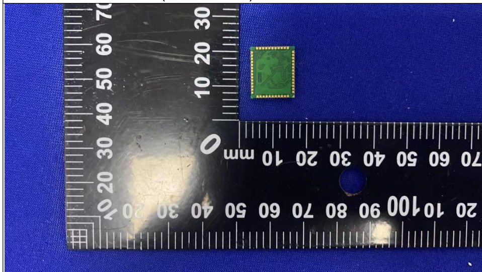
Model(Two antennas):WF-U21DS-SSA2
