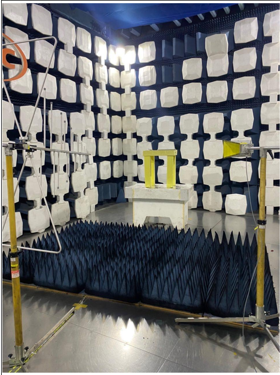
RADIATED SPURIOUS EMISSION TEST (ABOVE 1G)
