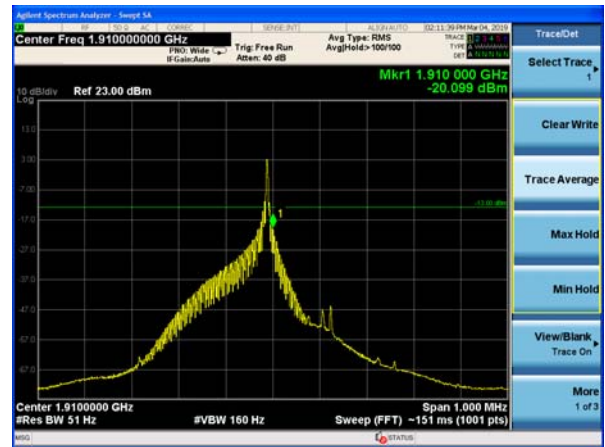
NB-IOT Band 2 QPSK 15kHz 1@0 CH-High
