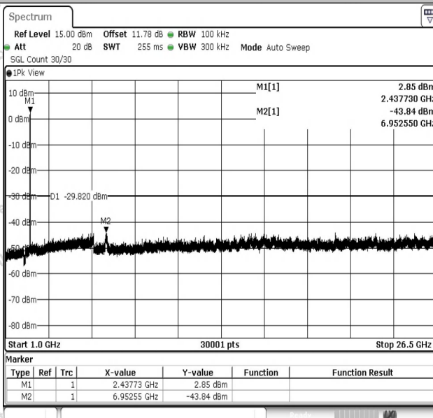
11B-Ant1-2437-1000~26500-PASS
