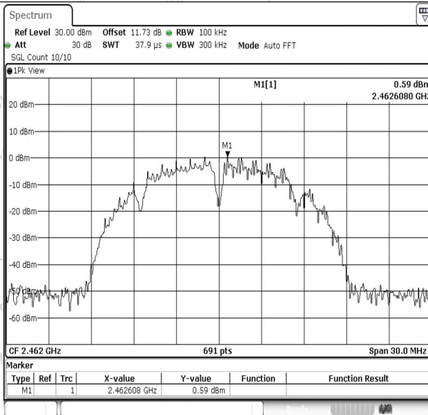
11B-Ant1-2462-0~Reference-PASS
