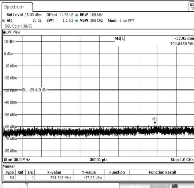
11B-Ant1-2462-30~1000-PASS
