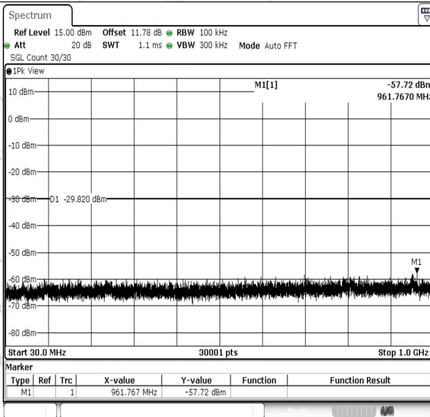
11B-Ant1-2437-30~1000-PASS
