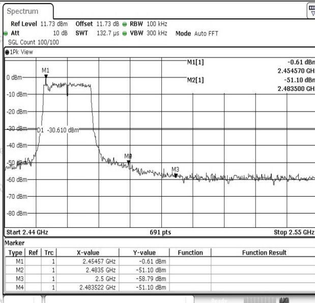
11G-Ant1-2462-PASS
