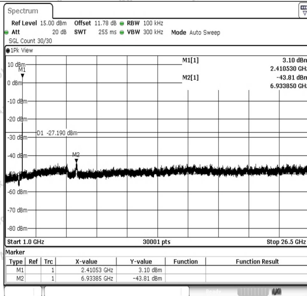
11B-Ant1-2412-1000~26500-PASS
