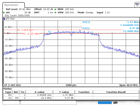
g_2462MHz_Chain 0
