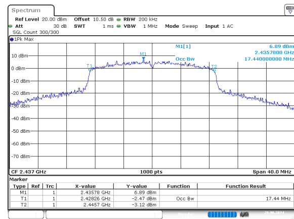
n20_2437MHz_Chain 0
