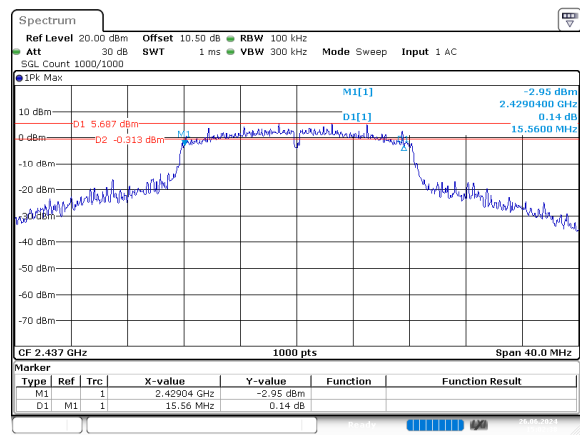
g_2437MHz_Chain 0
