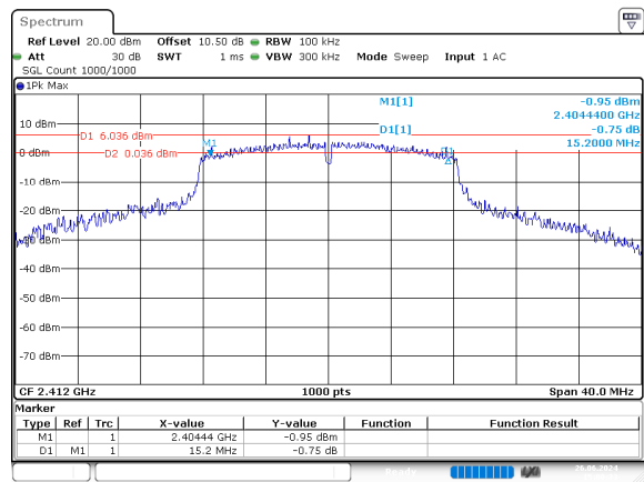
g_2412MHz_Chain 0
