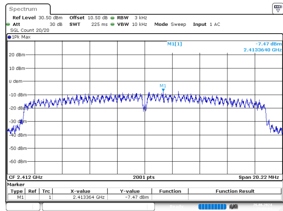
n20_2412MHz_Chain 0
