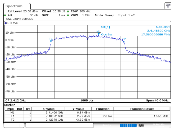
n20_2412MHz_Chain 0
