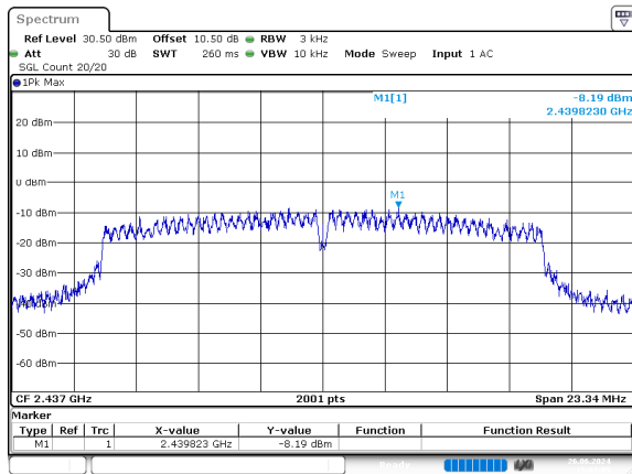
g_2437MHz_Chain 0
