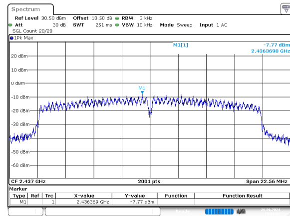
n20_2437MHz_Chain 0
