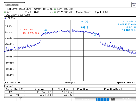
n20_2437MHz_Chain 0
