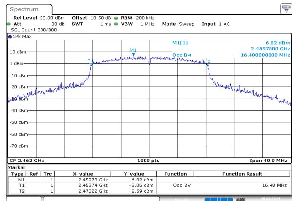
g_2462MHz_Chain 0
