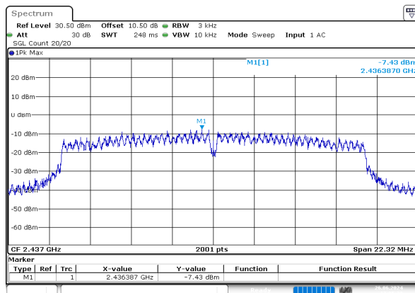
g_2437MHz_Chain 0
