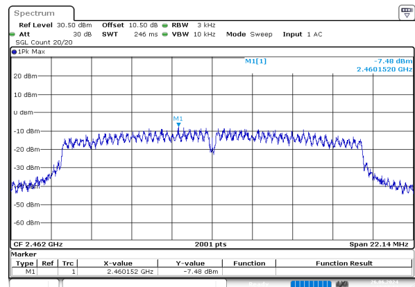
g_2462MHz_Chain 0
