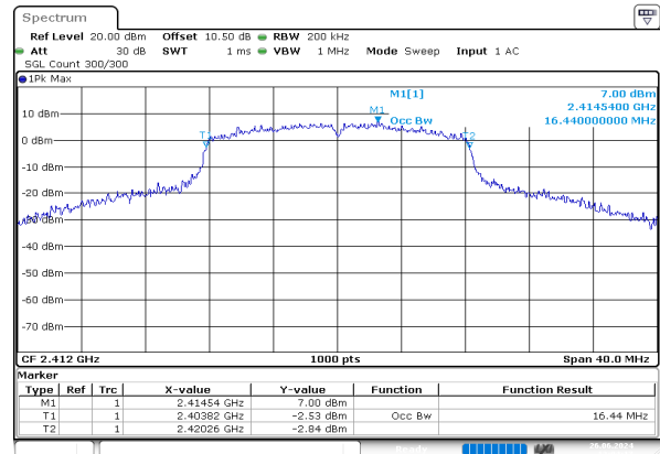
g_2412MHz_Chain 0
