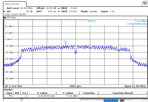
g_2412MHz_Chain 0
