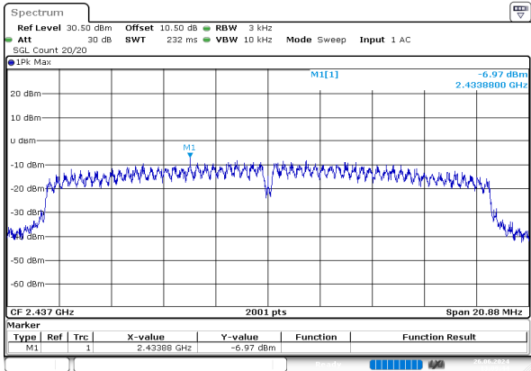
n20_2437MHz_Chain 0
