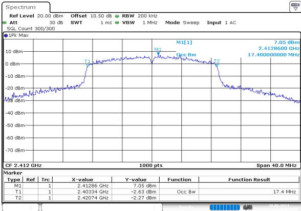
n20_2412MHz_Chain 0
