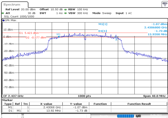
n20_2437MHz_Chain 0
