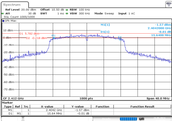
n20_2412MHz_Chain 0
