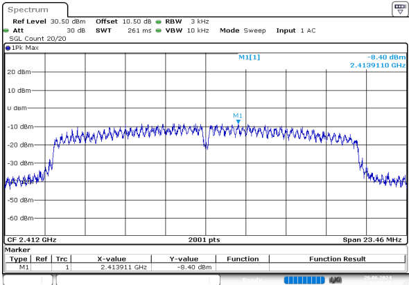
n20_2412MHz_Chain 0
