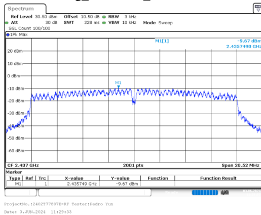
g_2437MHz_Chain 0
