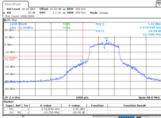
g_2412MHz_Chain 0
