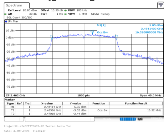
g_2462MHz_Chain 0
