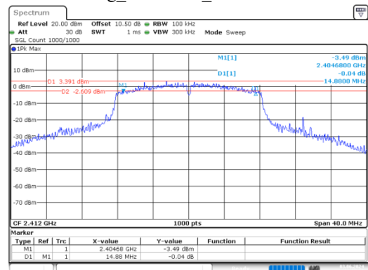
g_2412MHz_Chain 0
