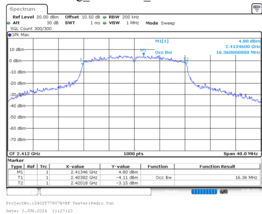
g_2412MHz_Chain 0
