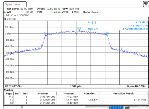
n20_2437MHz_Chain 0
