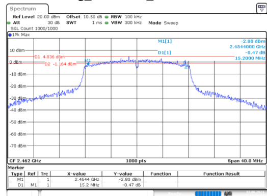
g_2462MHz_Chain 0
