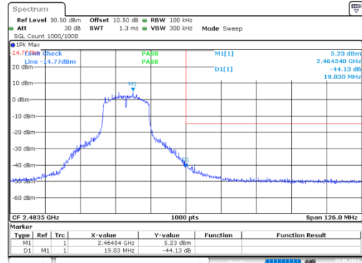
g_2462MHz_Chain 0
