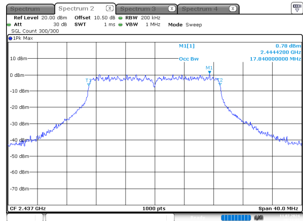
n20_2437MHz_Chain 0
