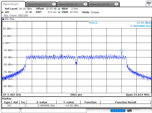
g_2462MHz_Chain 0
