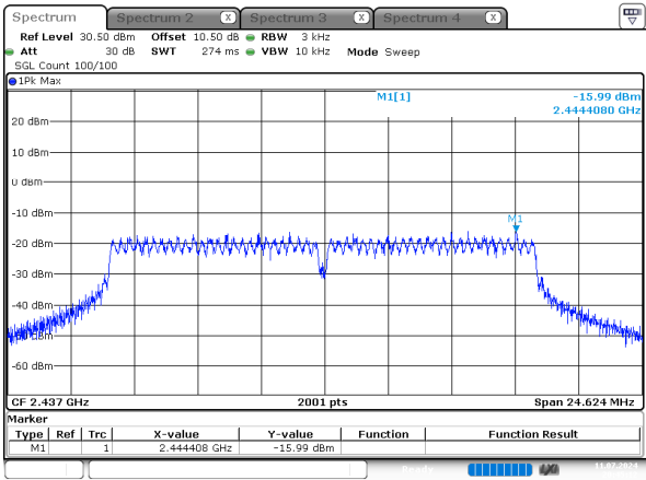
g_2437MHz_Chain 0
