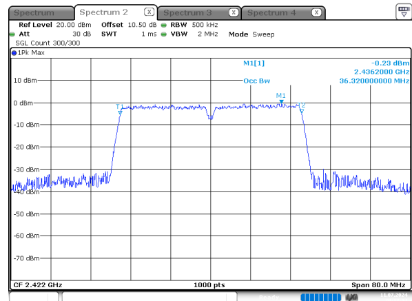
n40_2422MHz_Chain 0
