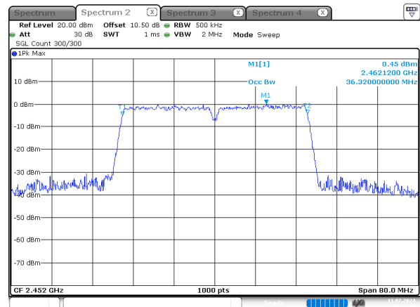
n40_2452MHz_Chain 0
