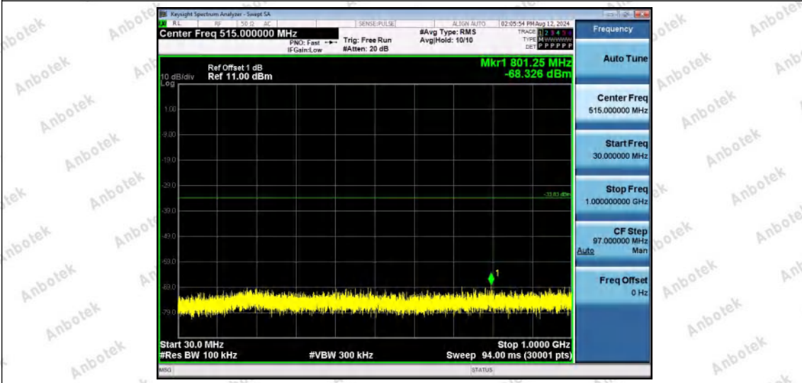
11N40SISO-Ant1-2452-30~1000-PASS
