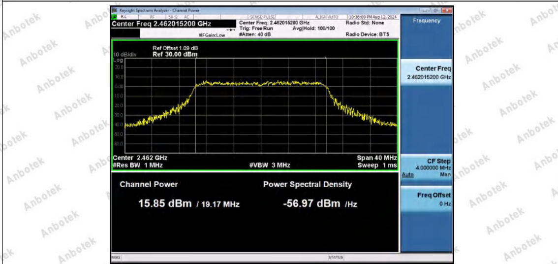
11AX20SISO-Ant1-2462-PASS
