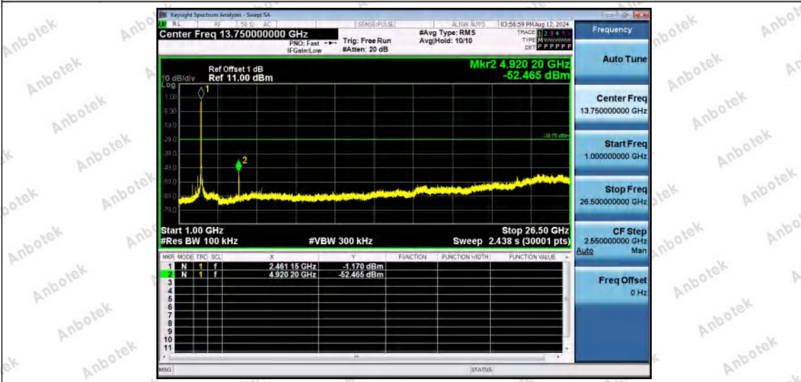
11AX20SISO-Ant1-2462-1000~26500-PASS
