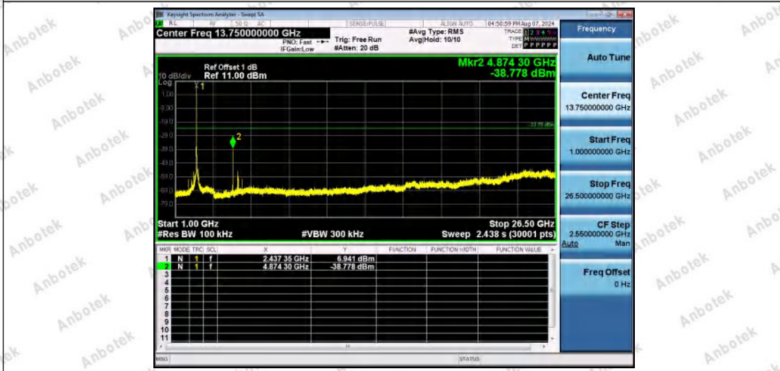
11B-Ant1-2437-1000~26500-PASS
