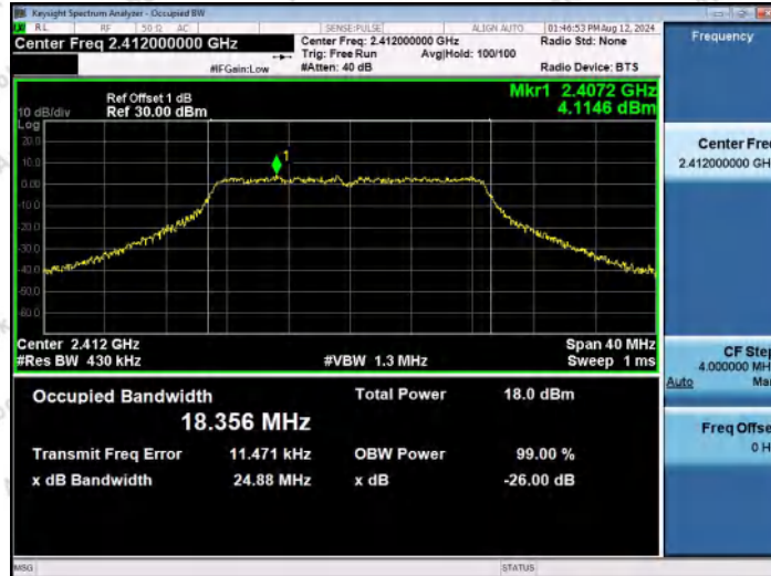
11N20SISO-Ant1-2412
