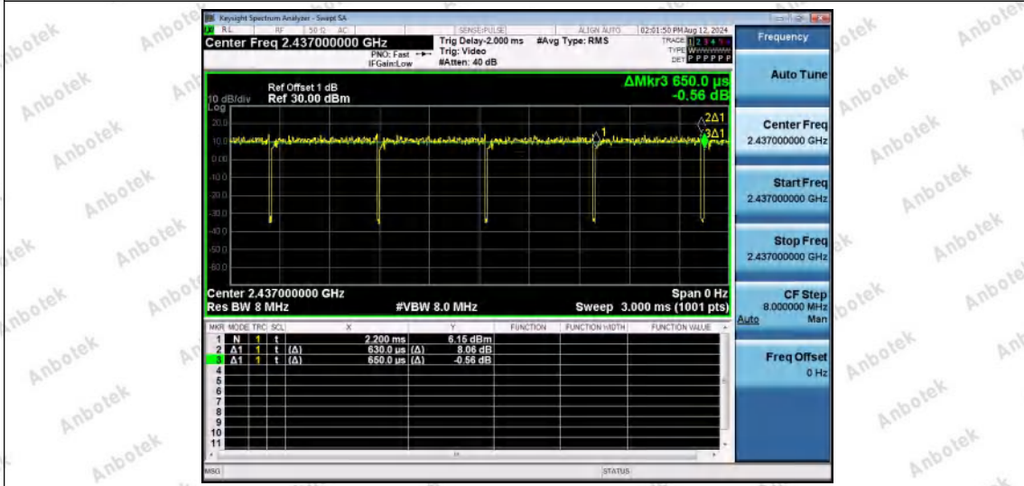
NTNV-11N40SISO-Ant1-2437
