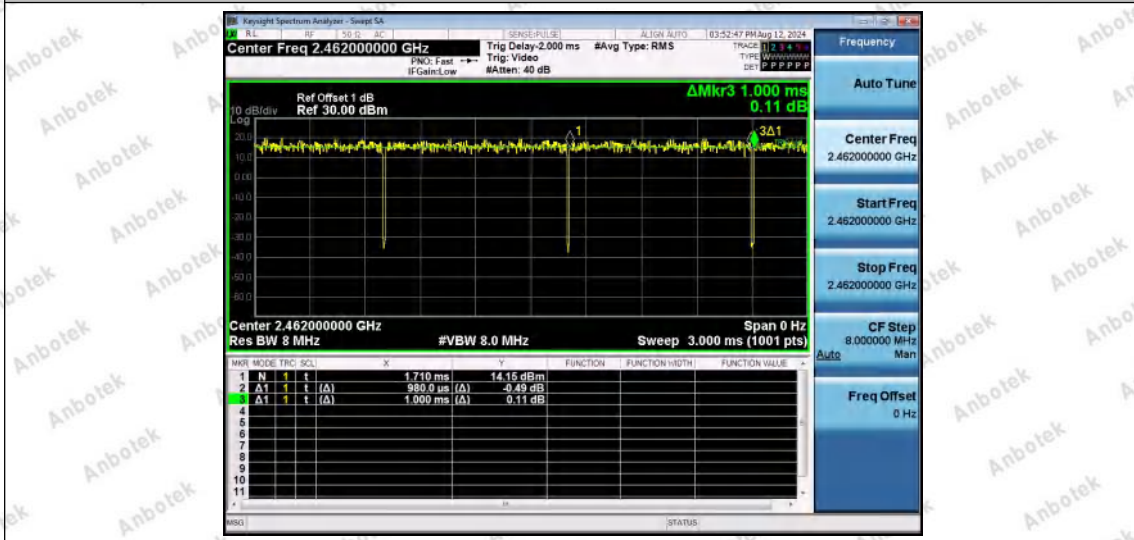
NTNV-11AX20SISO-Ant1-2462
