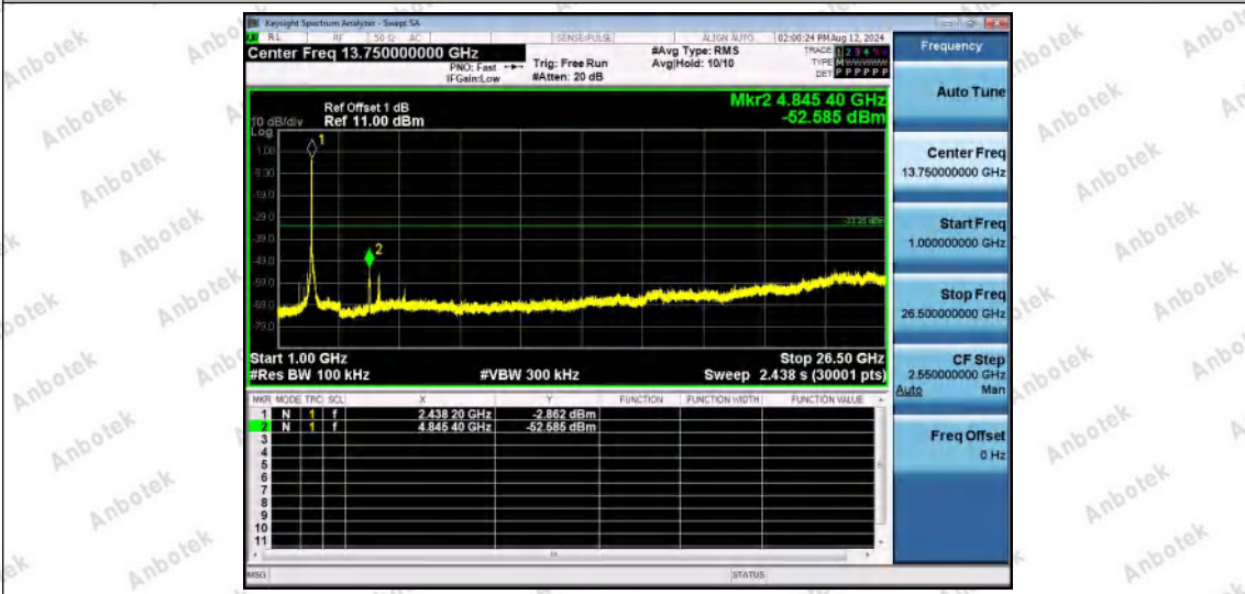
11N40SISO-Ant1-2422-1000~26500-PASS
