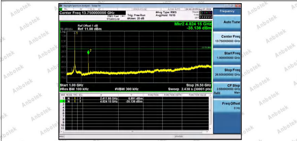
11B-Ant1-2412-1000~26500-PASS
