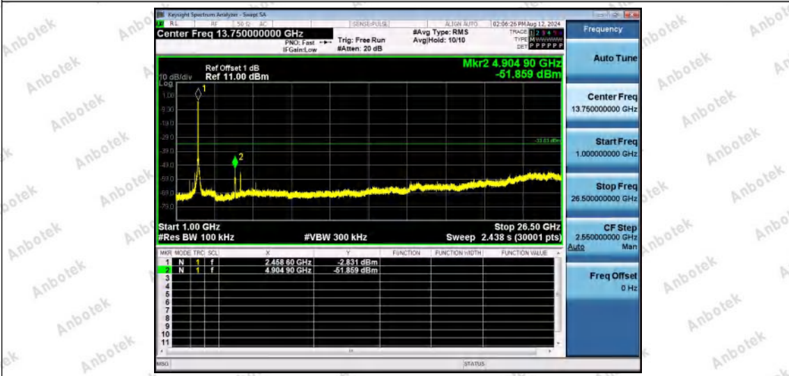
11N40SISO-Ant1-2452-1000~26500-PASS
