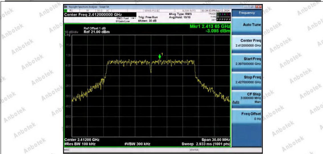
11G-Ant1-2412-0~Reference-PASS
