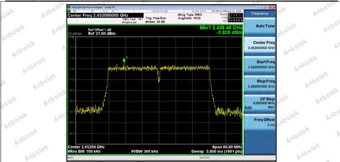
11N40SISO-Ant1-2452-0~Reference-PASS
