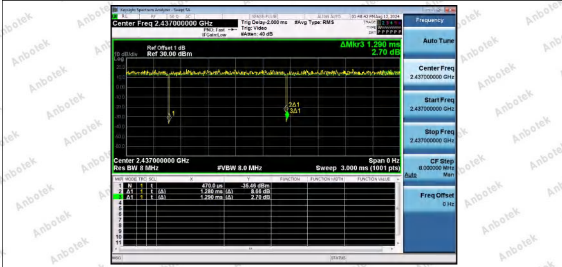
NTNV-11N20SISO-Ant1-2437
