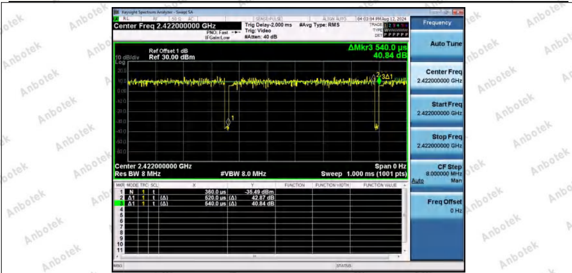
NTV-11AX40SISO-Ant1-2422
