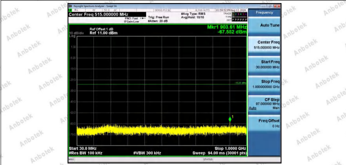
11N40SISO-Ant1-2422-30~1000-PASS
