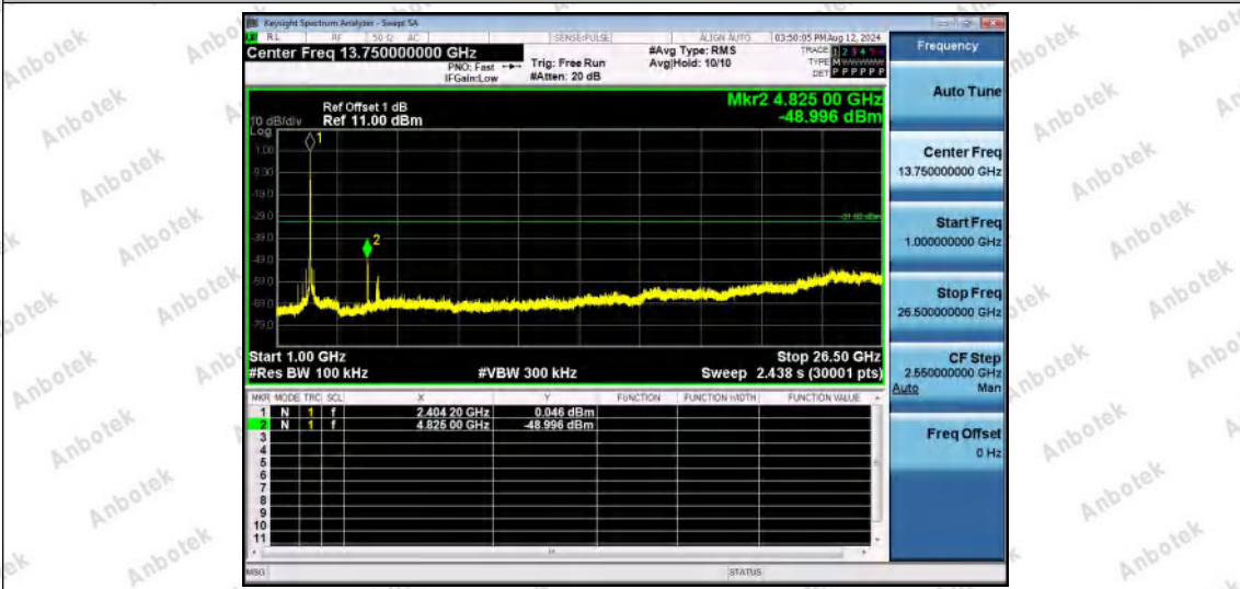
11AX20SISO-Ant1-2412-1000~26500-PASS
