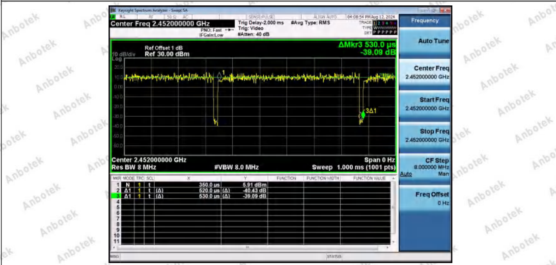
NTV-11AX40SISO-Ant1-2452
