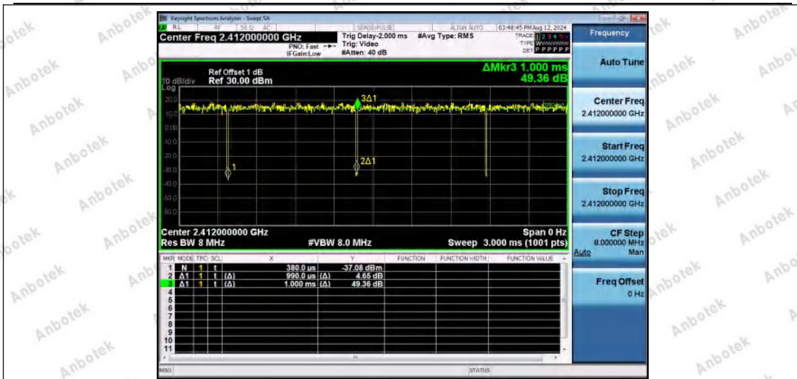
NTNV-11AX20SISO-Ant1-2412
