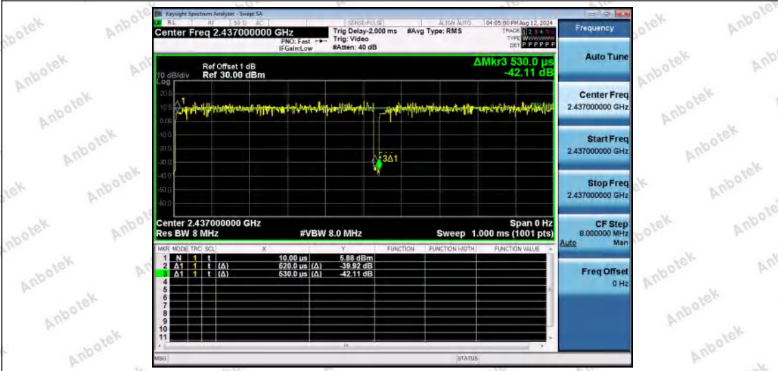
NTV-11AX40SISO-Ant1-2437
