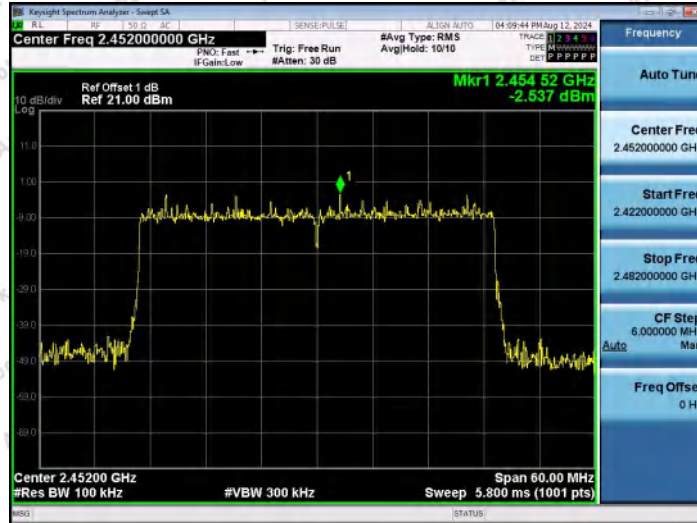
11AX40SISO-Ant1-2452-0~Reference-PASS
