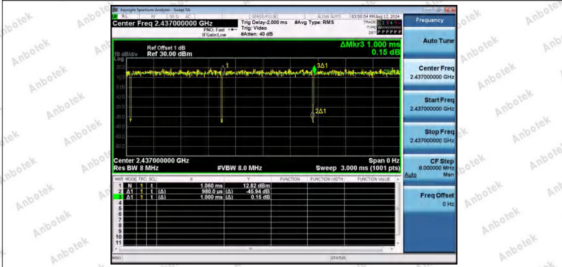
NTNV-11AX20SISO-Ant1-2437
