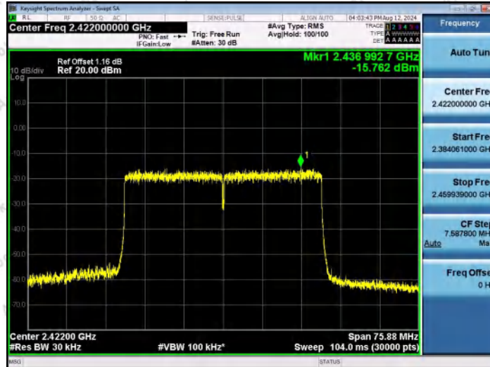
11AX40SISO-Ant1-2422-PASS
