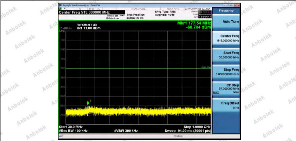
11N20SISO-Ant1-2437-30~1000-PASS
