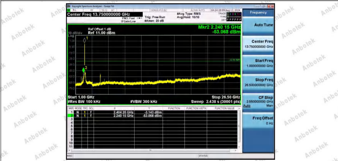
11AX40SISO-Ant1-2422-1000~26500-PASS
