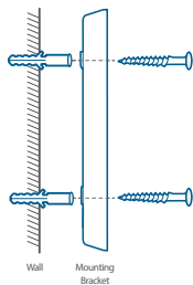
Without 15° Mounting Wedge
