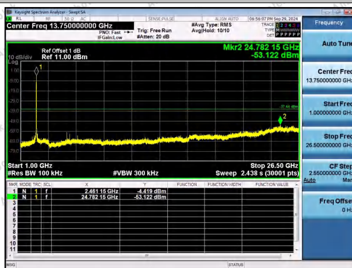
11N20SISO-Ant1-2462-1000~26500-PASS
