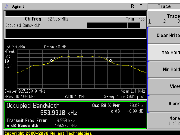
6dB Bandwidth plot on channel 03
