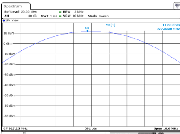
Peak output Power plot on channel 03
