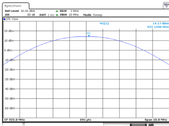
Peak output Power plot on channel 02
