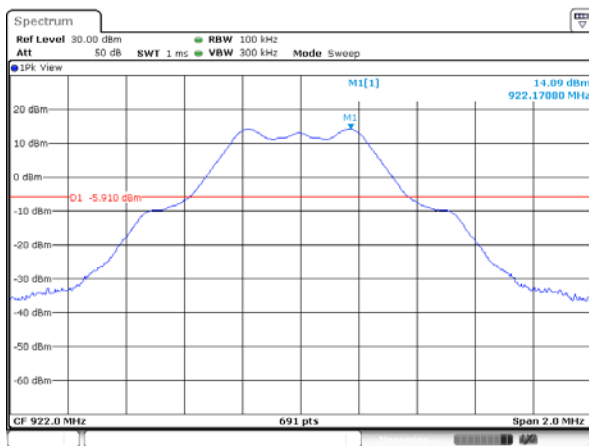
GFSK on channel 02
