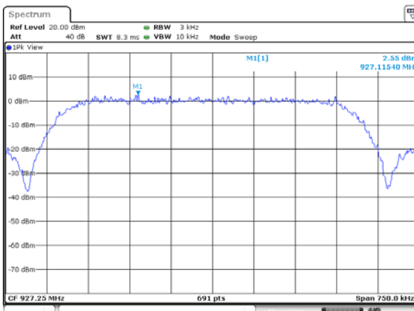
Power spectral density plot on channel 03
