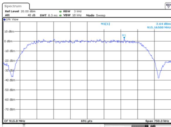
Power spectral density plot on channel 01
