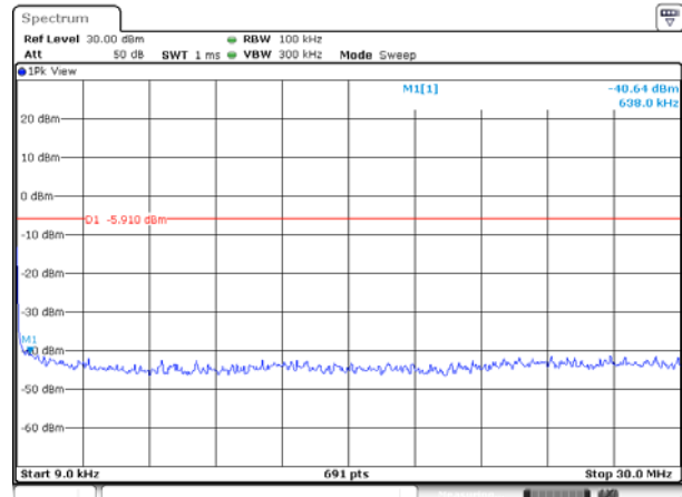
GFSK on channel 02
