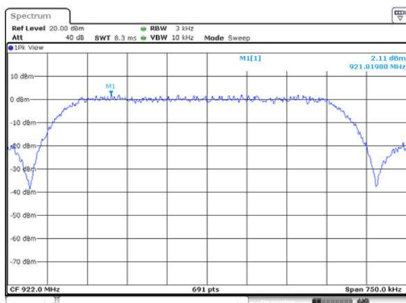
Power spectral density plot on channel 02
