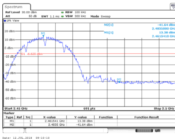
802.11b: Band Edge-High Channel
