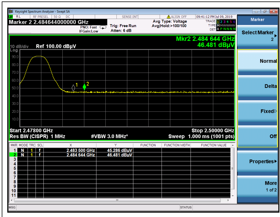
(Channel = 78, AVERAGE, π/4-DQPSK)
