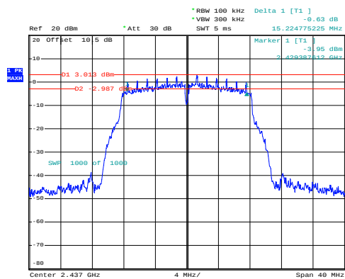
g_2437MHz_Chain 0
