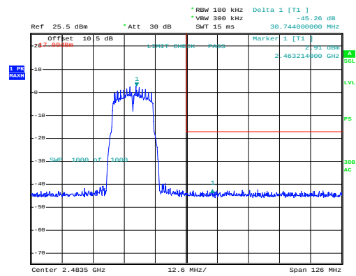
g_2462MHz_Chain 1
