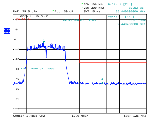
n40_2452MHz_Chain 1
