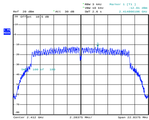
g_2412MHz_Chain 1
