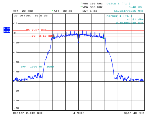
g_2412MHz_Chain 0
