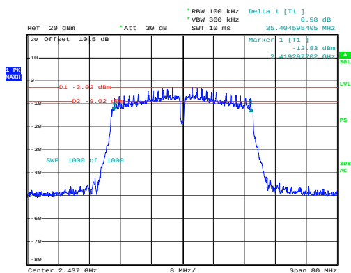
n40_2437MHz_Chain 0
