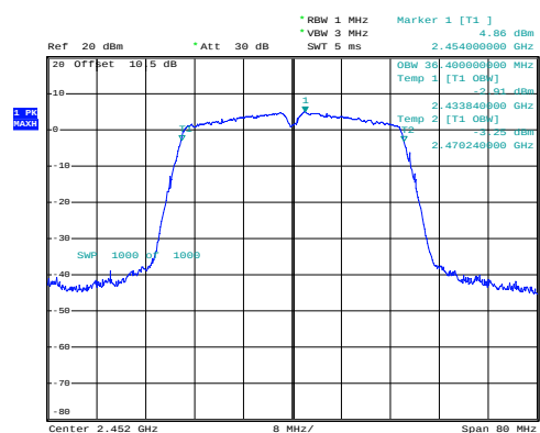
n40_2452MHz_Chain 0
