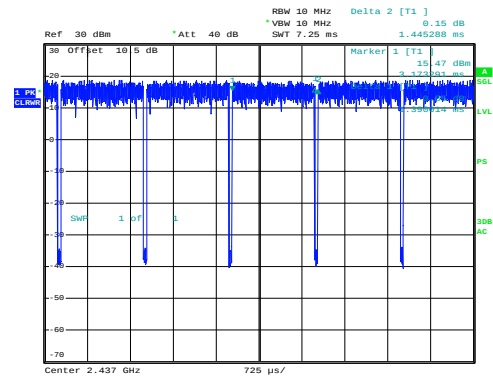
g_2437MHz_Chain 0
