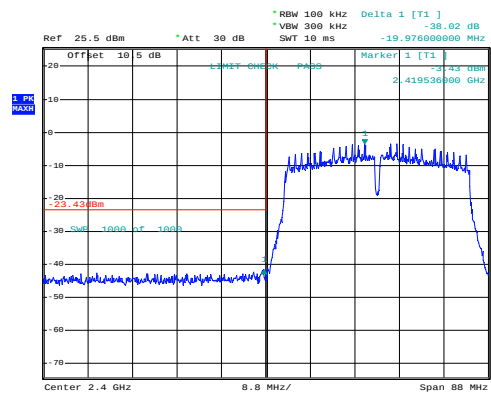
n40_2422MHz_Chain 1
