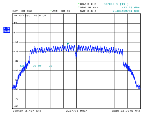
g_2437MHz_Chain 1
