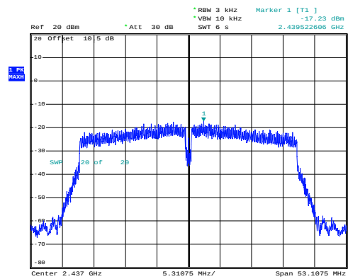
n40_2437MHz_Chain 1
