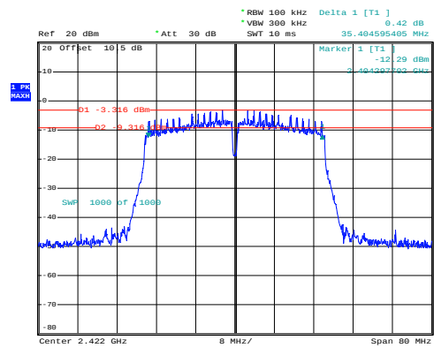
n40_2422MHz_Chain 0
