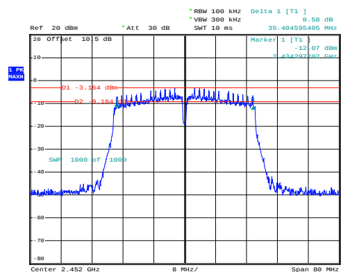
n40_2452MHz_Chain 0
