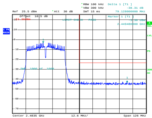
n40_2452MHz_Chain 0
