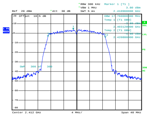
n20_2412MHz_Chain 0
