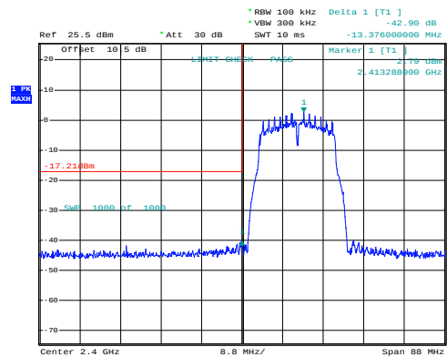
g_2412MHz_Chain 1
