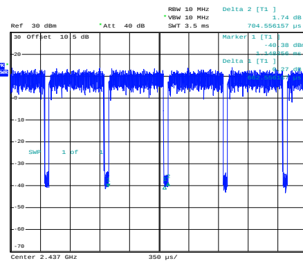
n40_2437MHz_Chain 0
