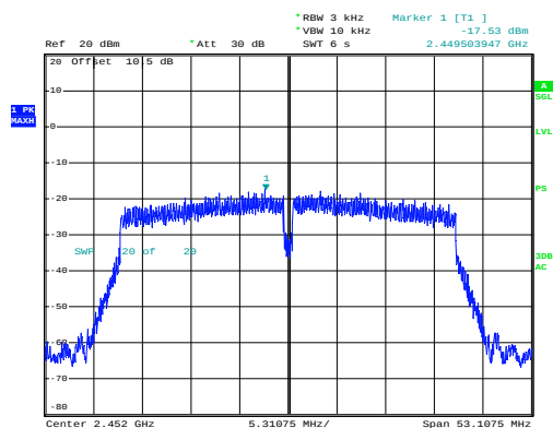
n40_2452MHz_Chain 0
