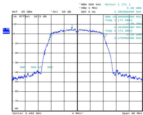
g_2462MHz_Chain 0
