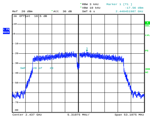
n40_2437MHz_Chain 0
