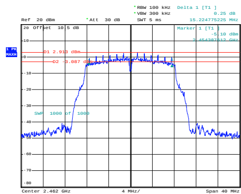
g_2462MHz_Chain 0
