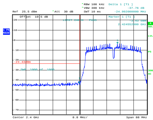
n40_2422MHz_Chain 0
