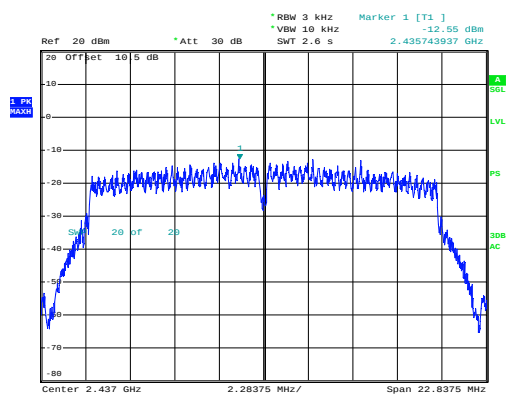
n20_2437MHz_Chain 0
