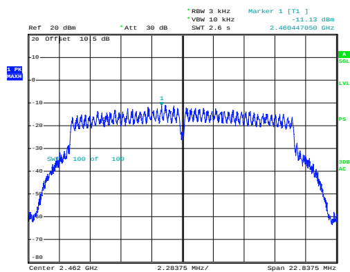
g_2462MHz_Chain 0 -
