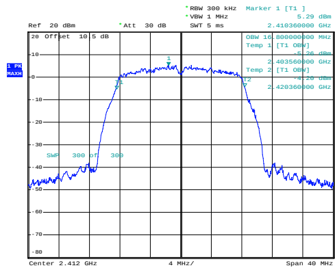
g_2412MHz_Chain 0
