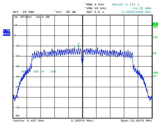
g_2437MHz_Chain 0
