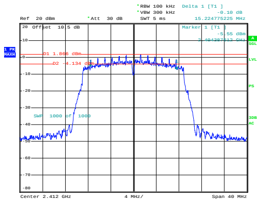
n20_2412MHz_Chain 0
