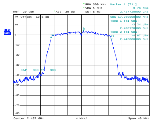
n20_2437MHz_Chain 0
