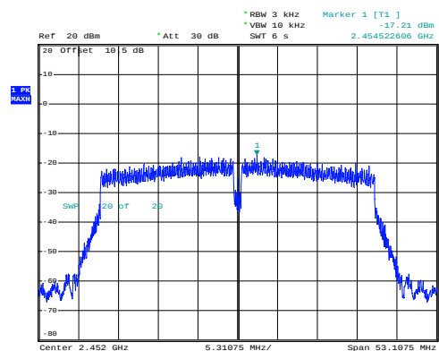
n40_2452MHz_Chain 1
