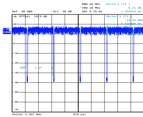
n20_2437MHz_Chain 0
