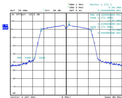
n40_2437MHz_Chain 0
