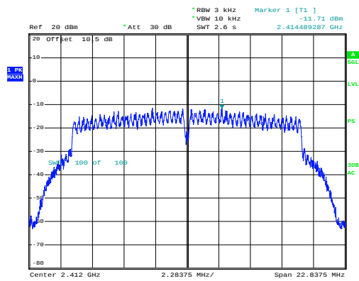
g_2412MHz_Chain 0
