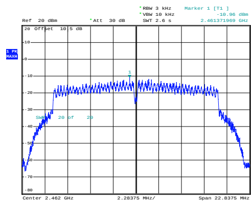
g_2462MHz_Chain 1
