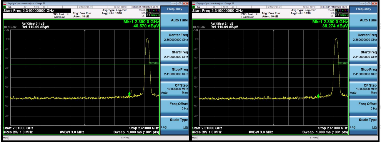
Peak Value(Vertical)
