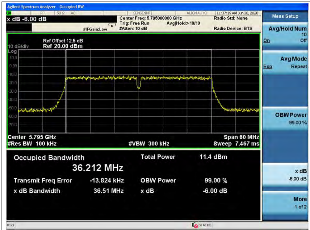
(Channel 159,5795MHz,802.11n(HT40))
