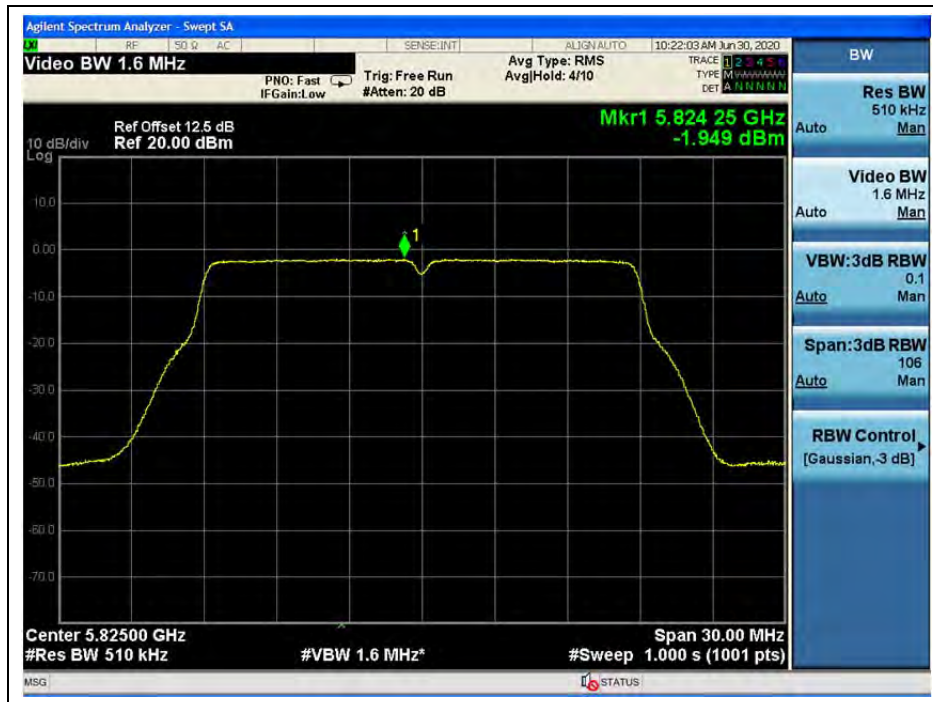
(Channel 165,5825MHz, 802.11ac (VHT20), ANT 1)
