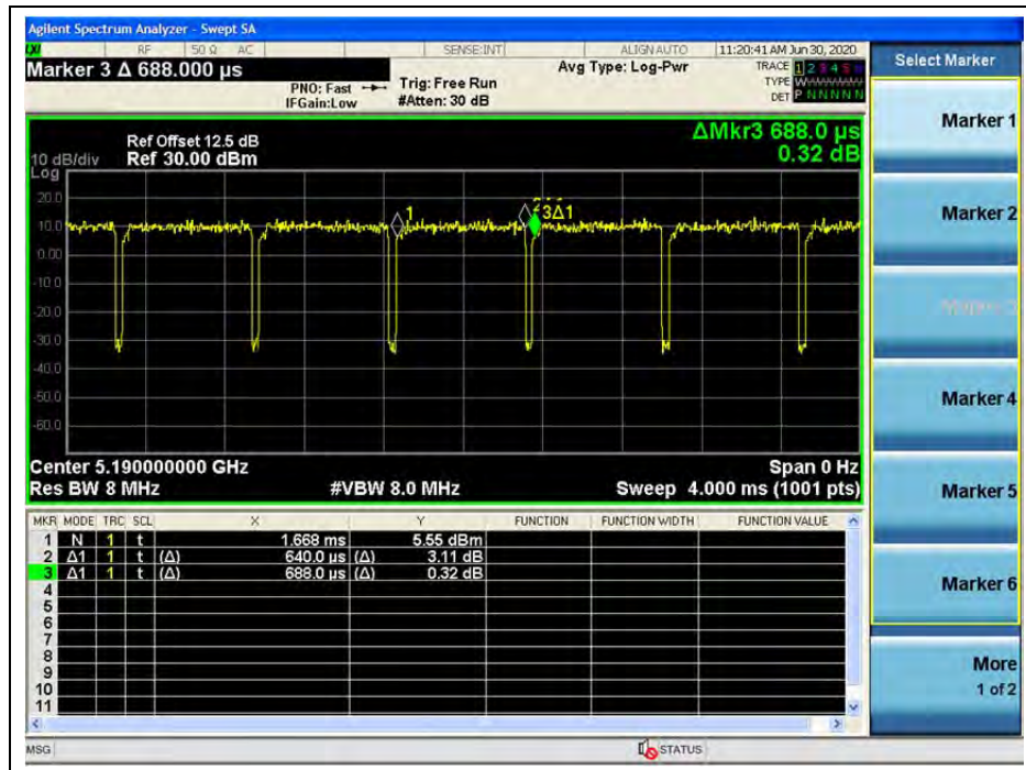
(CH38_5190MHz_802.11n(HT40))
