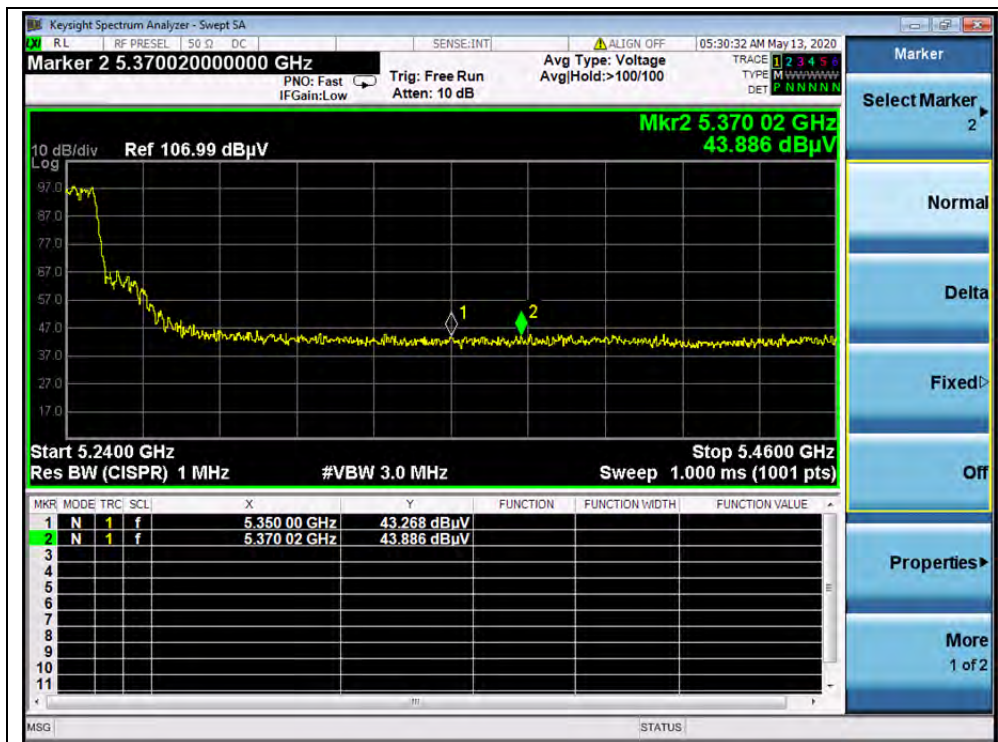
(PEAK, Channel 48, 802.11n (HT20))
