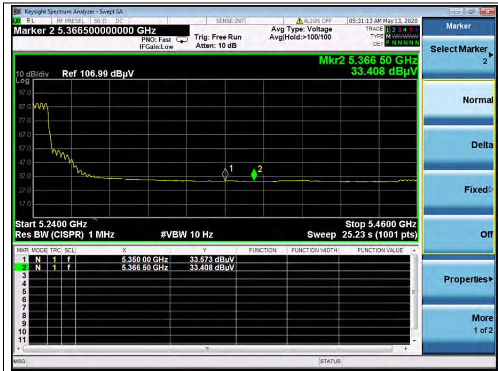
(AVG, Channel 48,802.11n (HT20))
