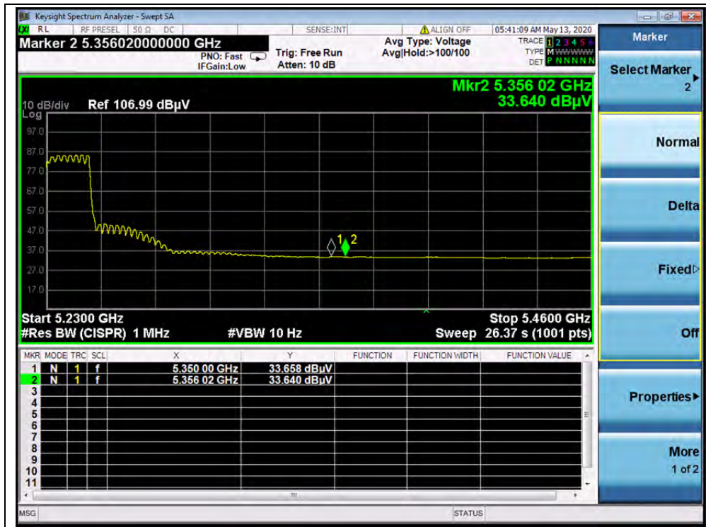
(AVG, Channel 46, 802.11ac (VHT40))
