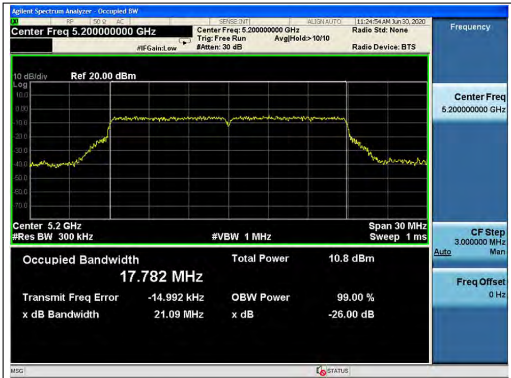
(Channel 40, 5200 MHz, 802.11n (HT20))
