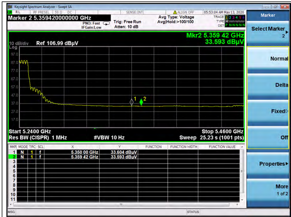
(AVG, Channel 48,802.11ac (VHT20))
