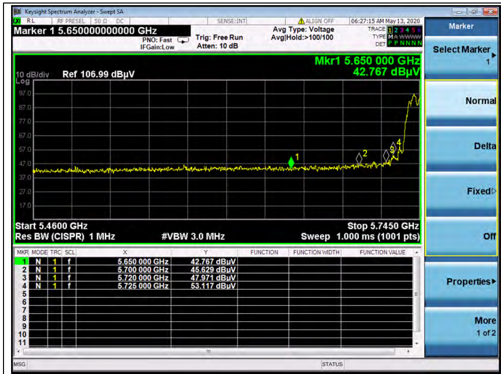
(PEAK, Channel 149, 802.11a)
