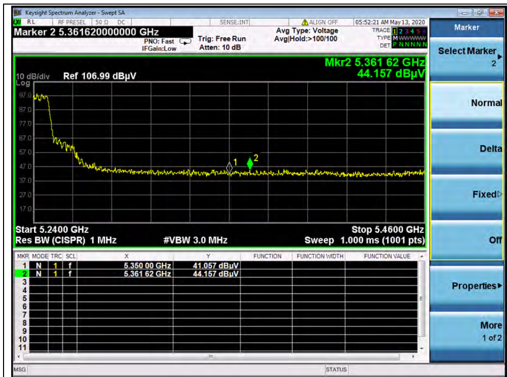
(PEAK, Channel 48, 802.11ac (VHT20))
