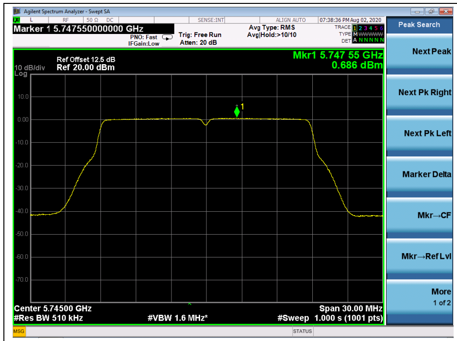
(Channel 149, 5745MHz, 802.11ac (VHT20), ANT R)
