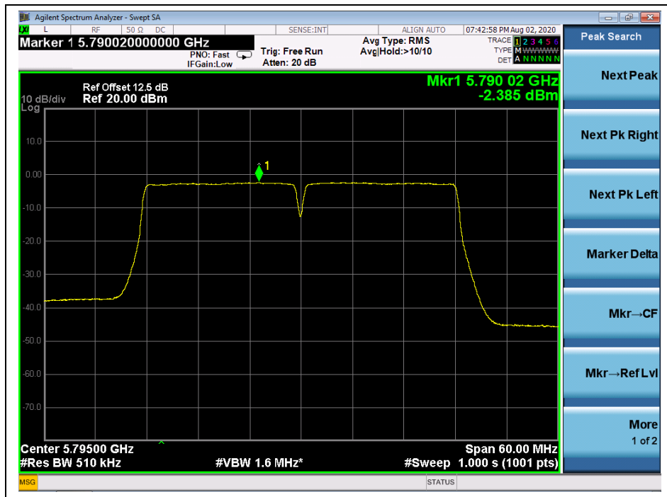
(Channel 159, 5795MHz, 802.11ac (VHT40), ANT R)
