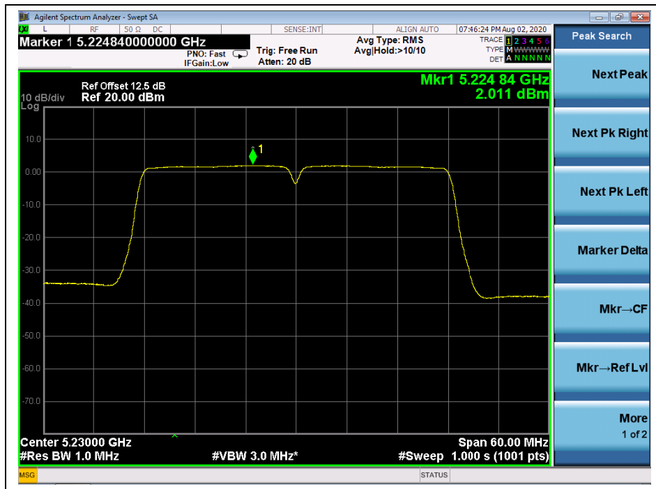
(Channel 46, 5230 MHz, 802.11n (HT40), ANT R)
