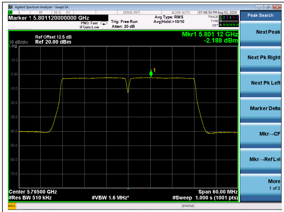
(Channel 159, 5795MHz, 802.11n (HT40), ANT R)
