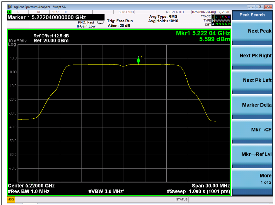
(Channel 44, 5220 MHz, 802.11a, ANT R)
