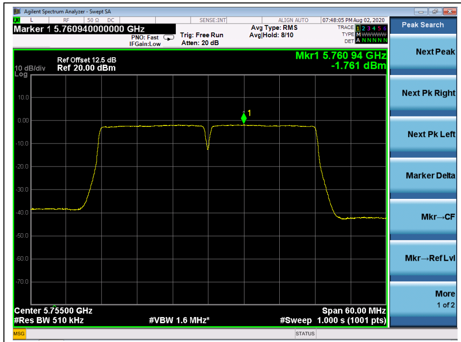
(Channel 151, 5755 MHz, 802.11n (HT40), ANT R)
