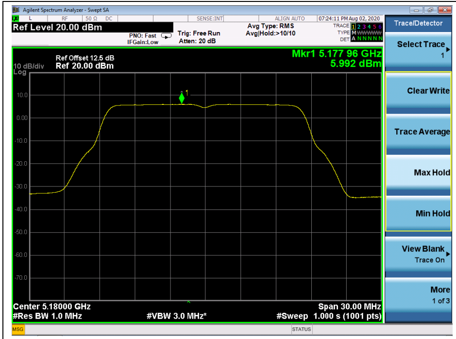
(Channel 36, 5180MHz, 802.11a, ANT R)
