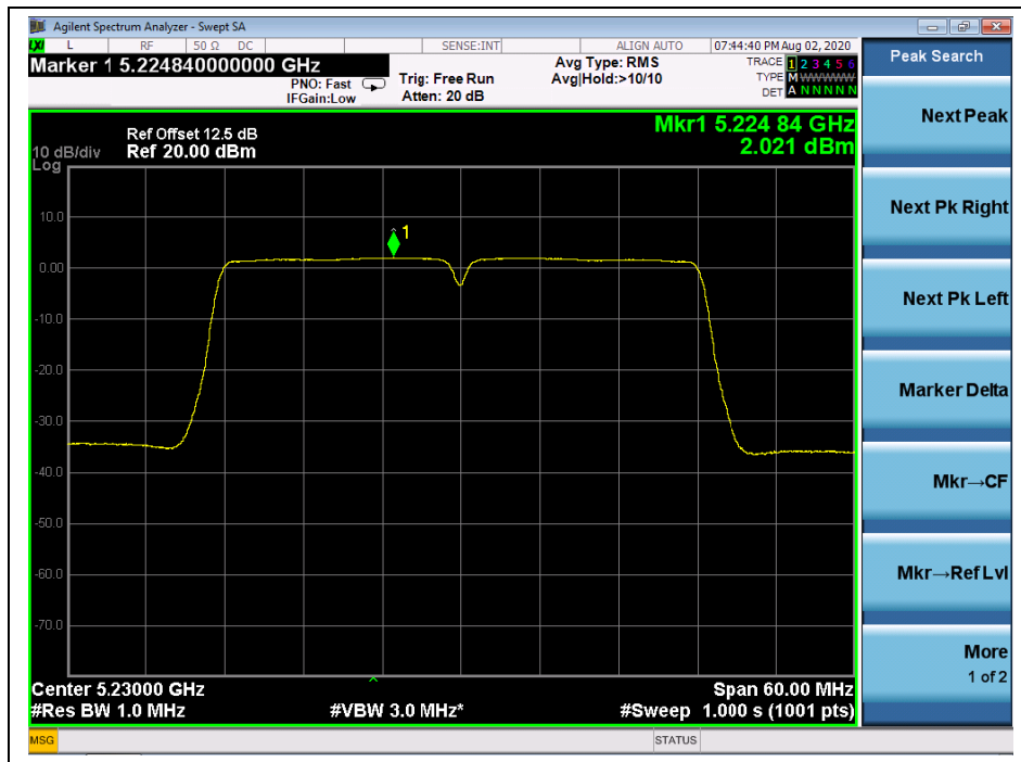
(Channel 46, 5230 MHz, 802.11ac (VHT40), ANT R)
