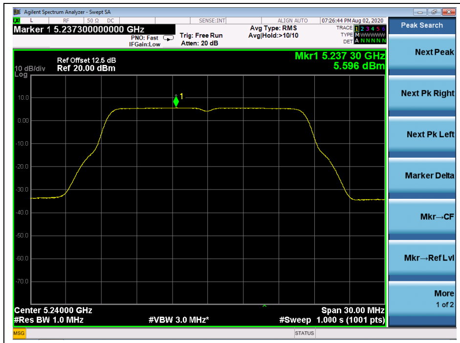
(Channel 48, 5240MHz, 802.11a, ANT R)
