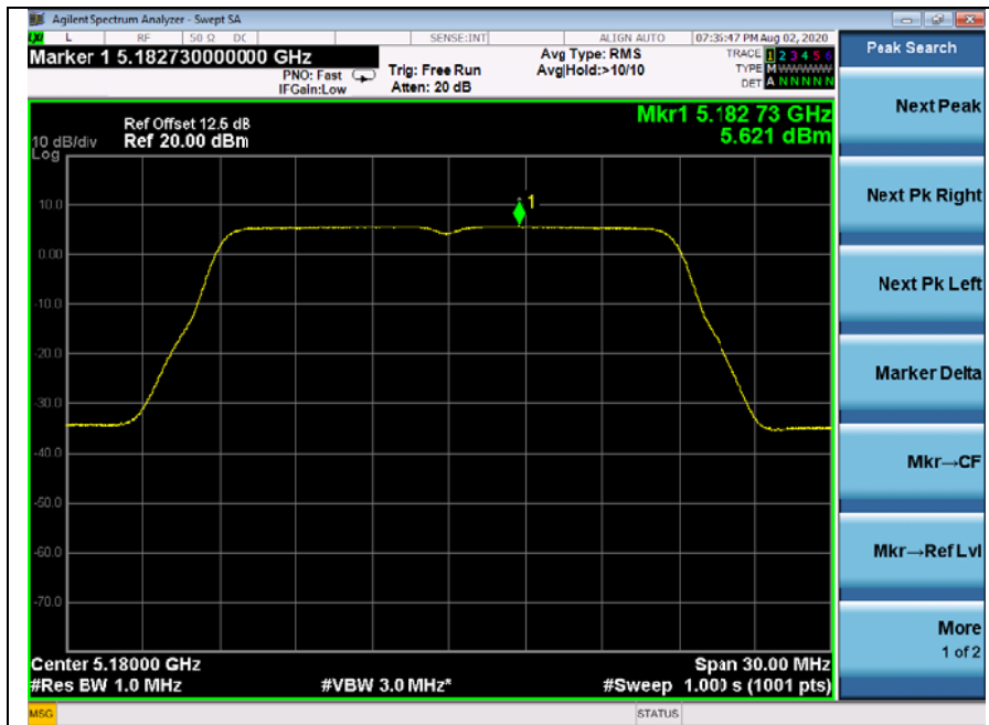
(Channel 36, 5180MHz, 802.11ac (VHT20), ANT R)
