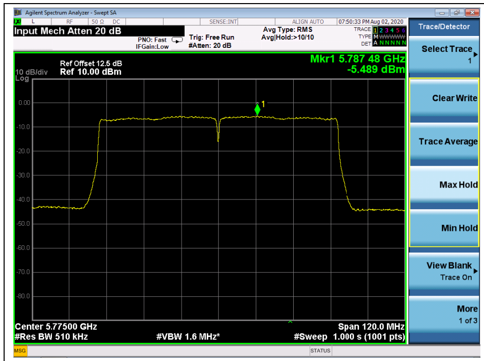
(Channel 155, 5775MHz, 802.11ac (VHT80), ANT R)
