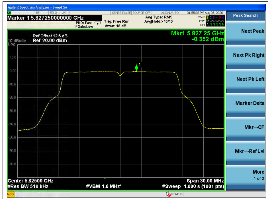
(Channel 165,5825MHz, 802.11a, ANT L)
