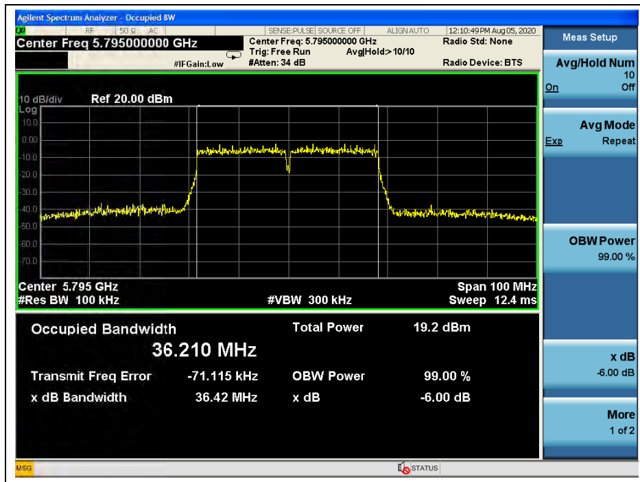
(Channel 159,5795MHz,802.11ac(VHT40))
