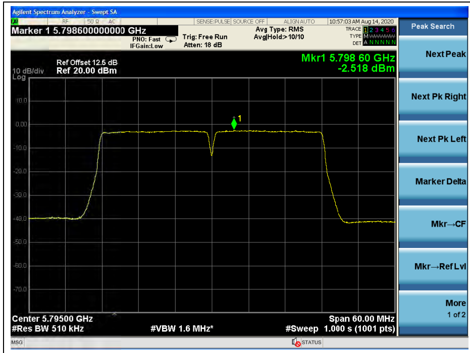
(Channel 159, 5795MHz, 802.11ac (VHT40), ANT R)
