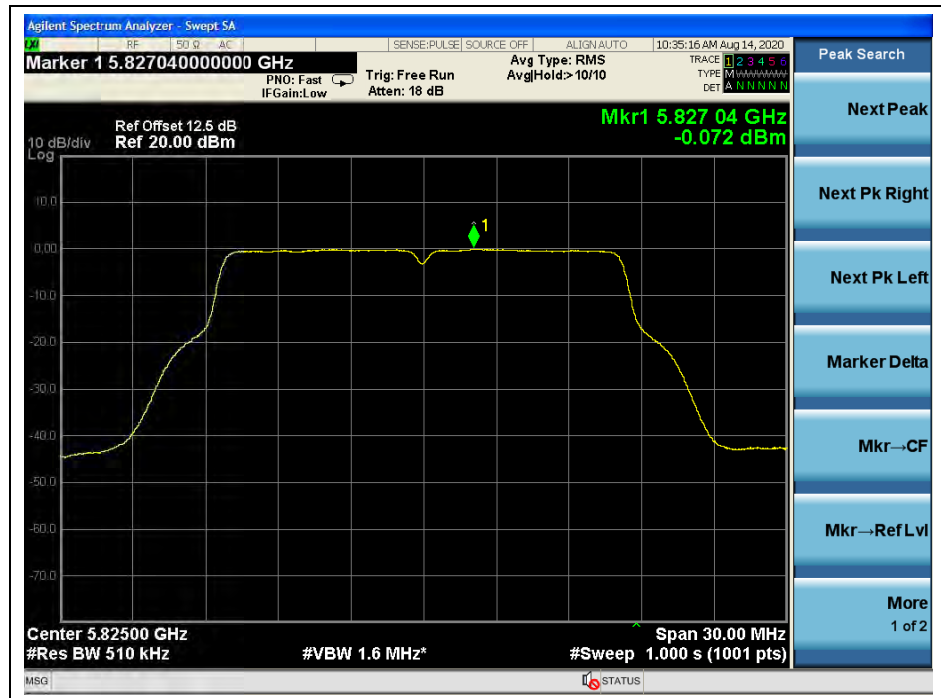
(Channel 165, 5825MHz, 802.11a, ANT R)
