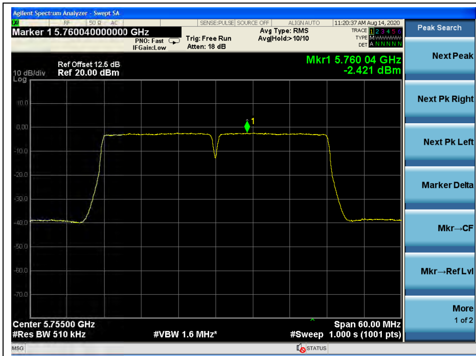
(Channel 151, 5755MHz, 802.11n (HT40), ANT R)
