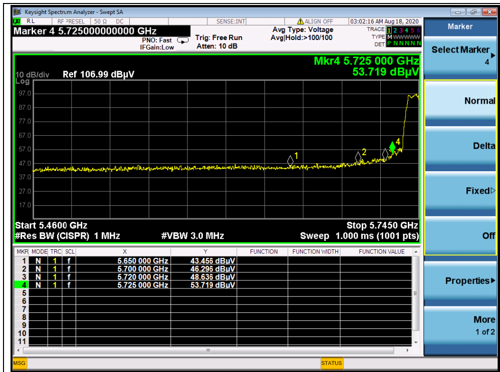
(PEAK,Channel 149, 802.11a)
