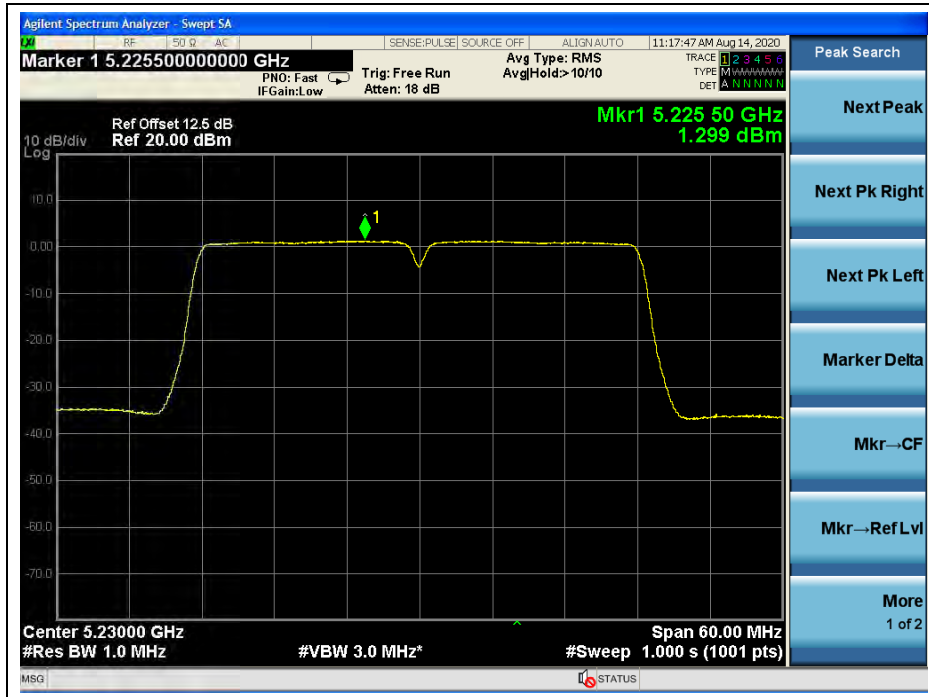
(Channel 46, 5230MHz, 802.11n (HT40), ANT R)
