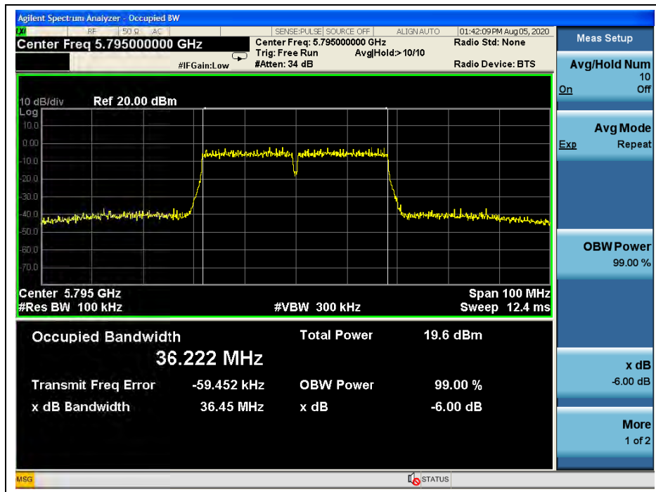
(Channel 159,5795MHz,802.11n(HT40))
