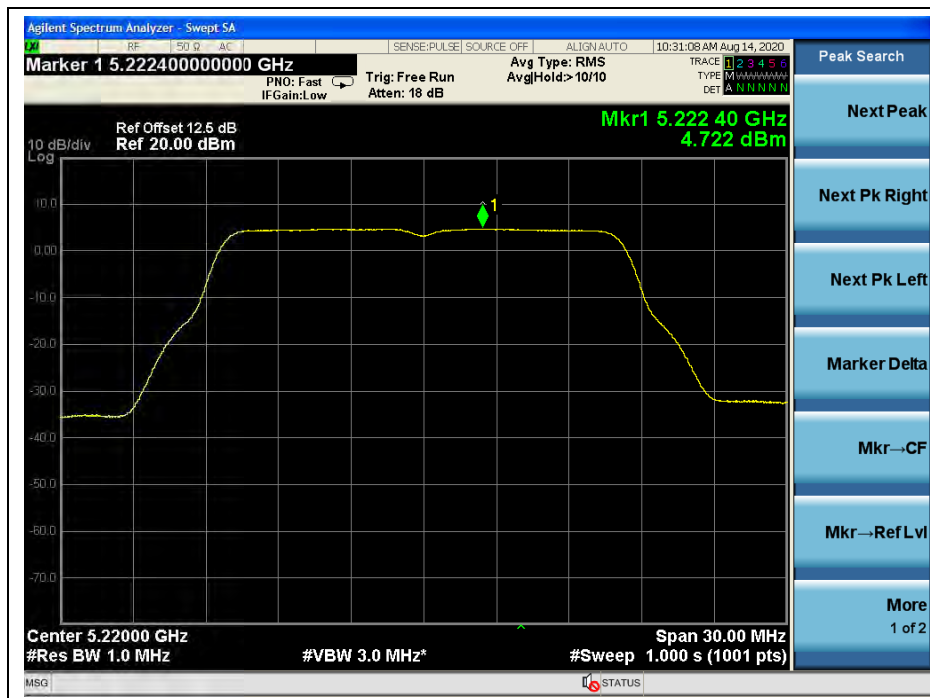
(Channel 44, 5220MHz, 802.11a, ANT R)
