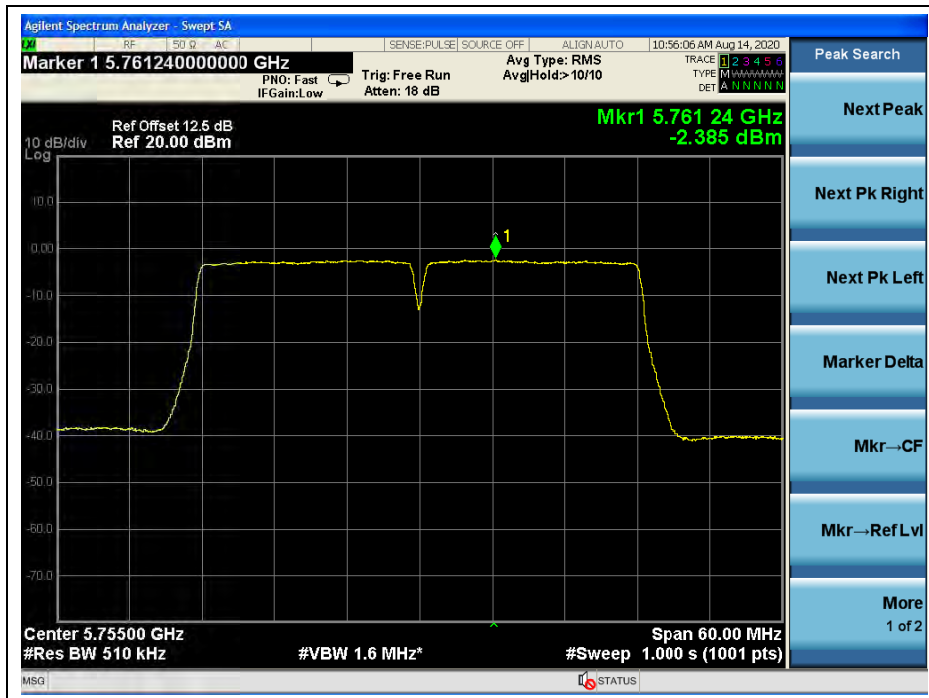
(Channel 151, 5755MHz, 802.11ac (VHT40), ANT R)
