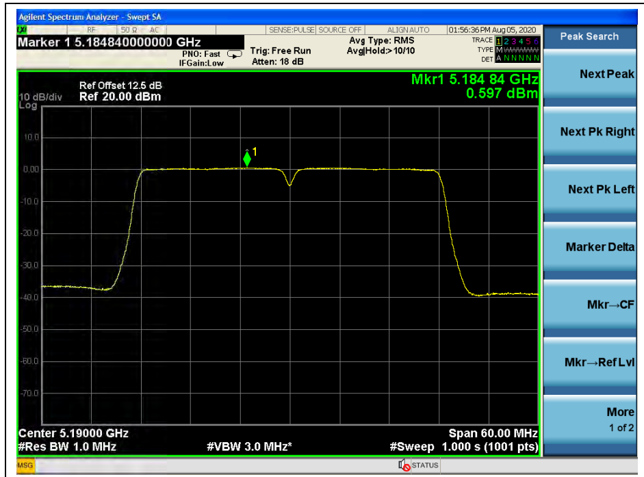
(Channel 38,5190MHz, 802.11n(HT40), ANT L)
