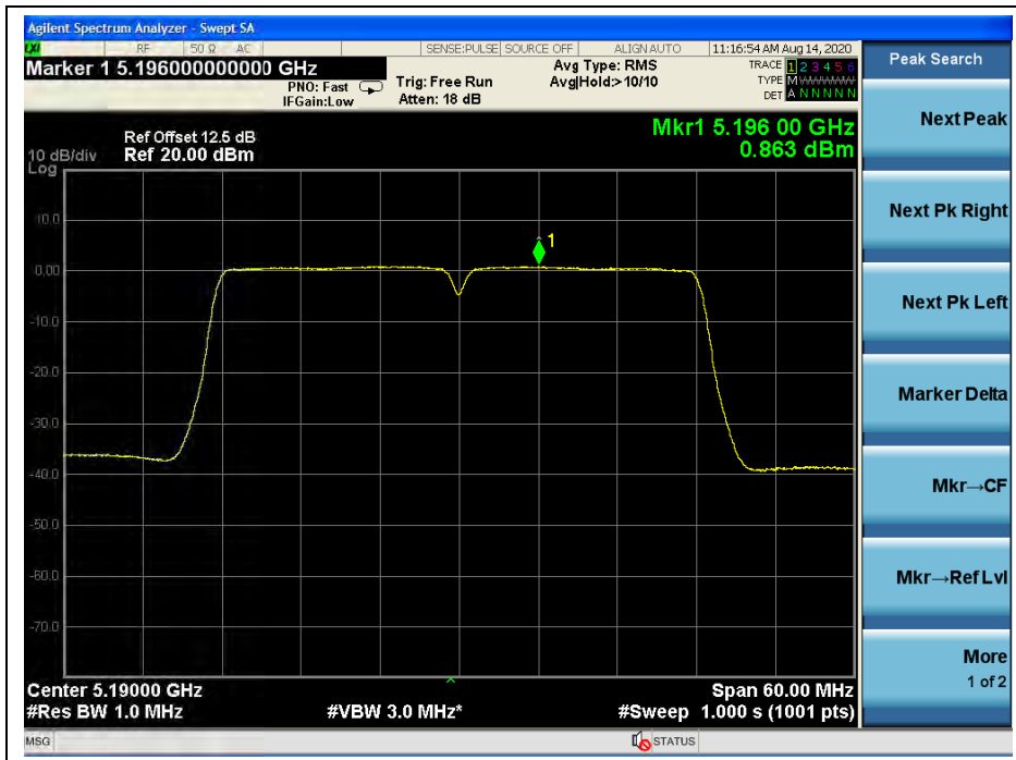
(Channel 38, 5190MHz, 802.11n (HT40), ANT R)
