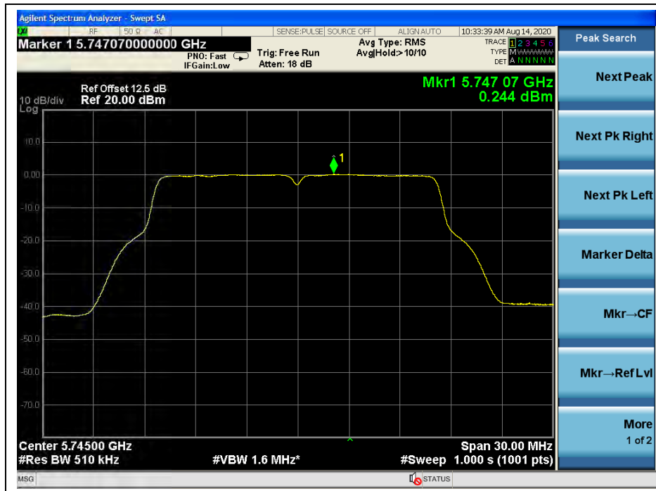
(Channel 149, 5745MHz, 802.11a, ANT R)
