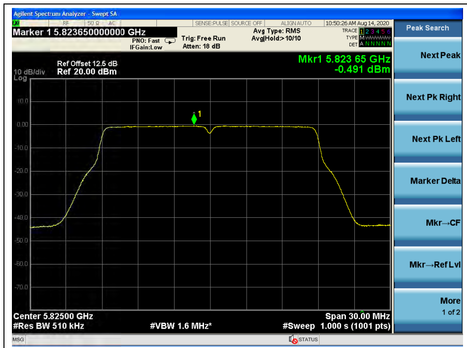
(Channel 165, 5825MHz, 802.11ac (VHT20), ANT R)
