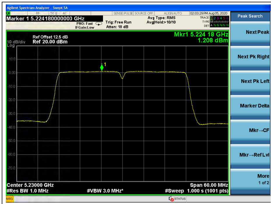
(Channel 46, 5230 MHz, 802.11ac (VHT40), ANT L)
