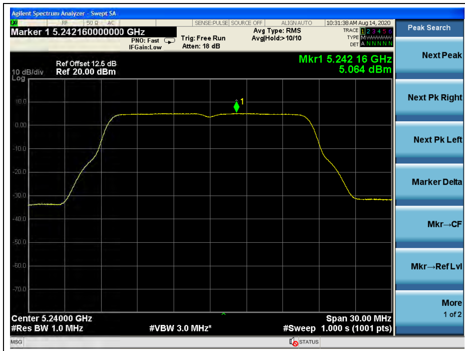
(Channel 48, 5240MHz, 802.11a, ANT R)
