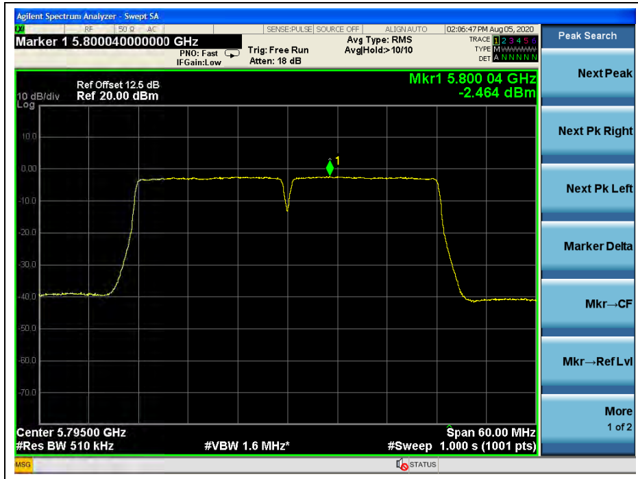
(Channel 159, 5795MHz, 802.11ac (VHT40), ANT L)
