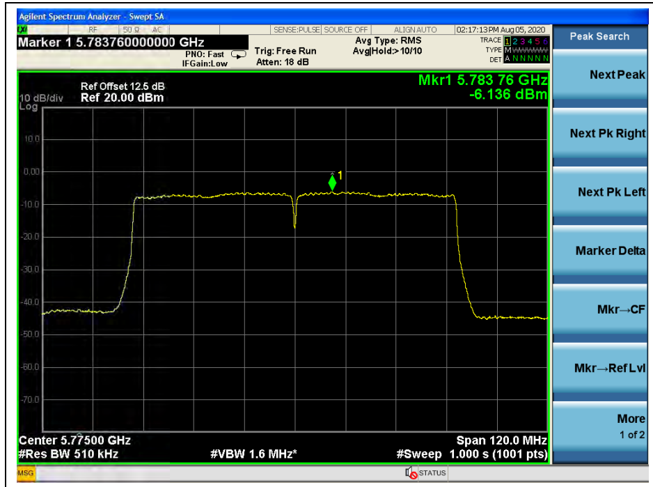
(Channel 155, 5775MHz, 802.11ac (VHT80), ANT L)
