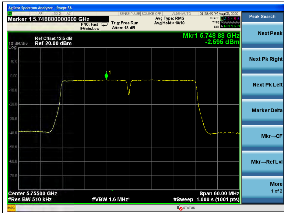
(Channel 151, 5755MHz, 802.11n (HT40), ANT L)
