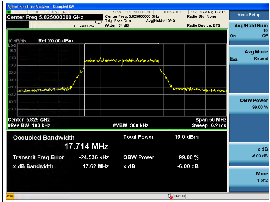
(Channel 165,5825MHz, 802.11 ac (VHT20))
