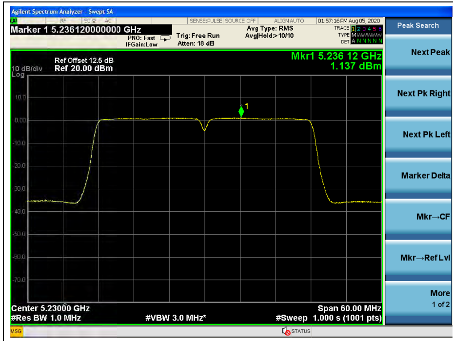
(Channel 46, 5230MHz, 802.11n(HT40), ANT L)
