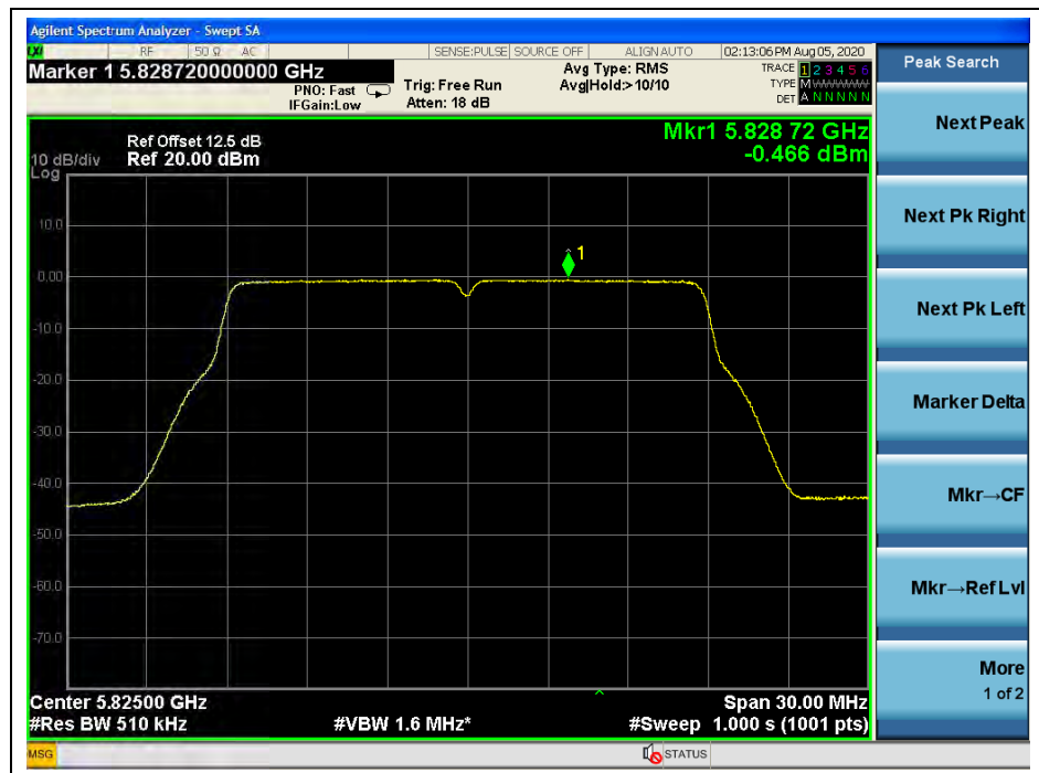
(Channel 165,5825MHz, 802.11n (HT20), ANT L)
