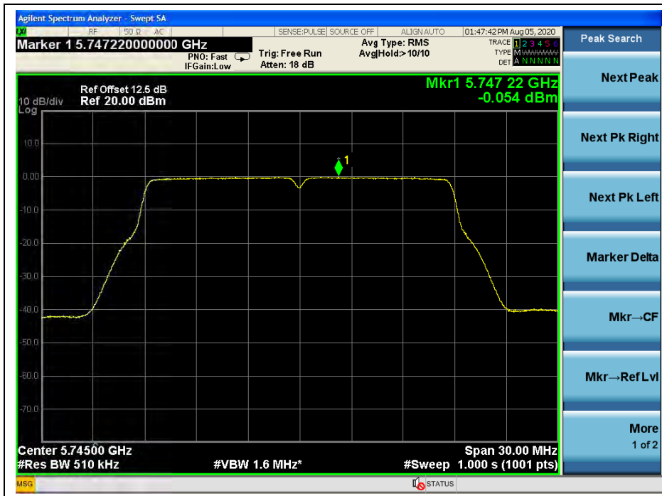
(Channel 149, 5745MHz, 802.11ac (VHT20), ANT L)
