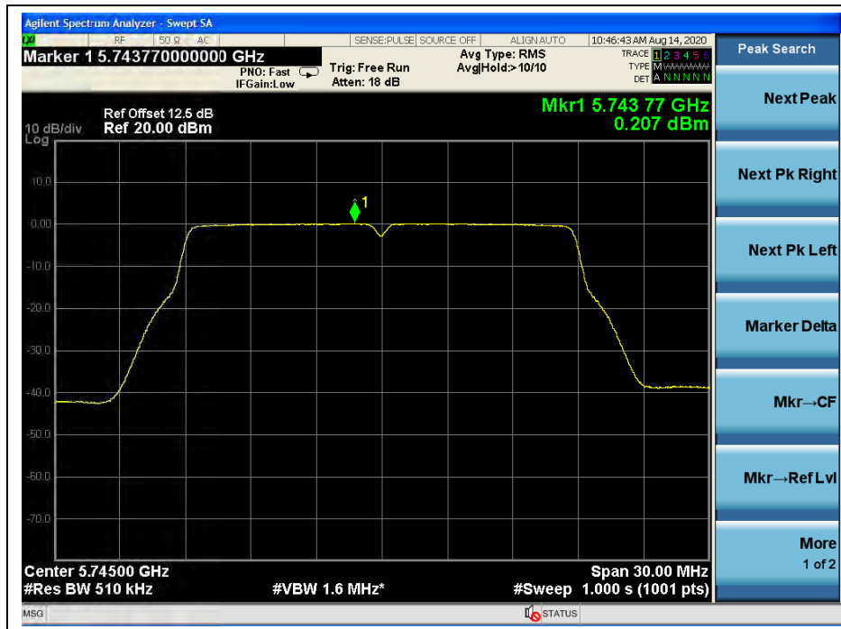
(Channel 149, 5745MHz, 802.11ac (VHT20), ANT R)
