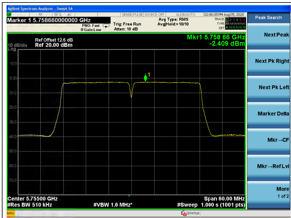
(Channel 151, 5755MHz, 802.11ac (VHT40), ANT L)
