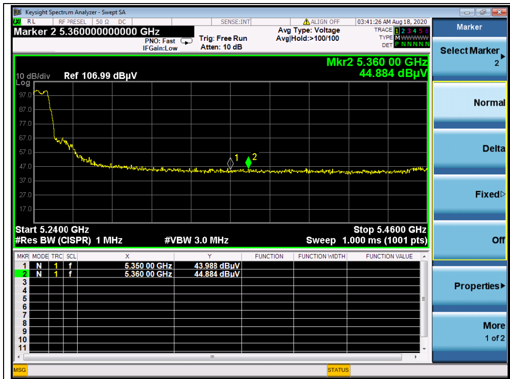
(PEAK,Channel 48, 802.11a)
