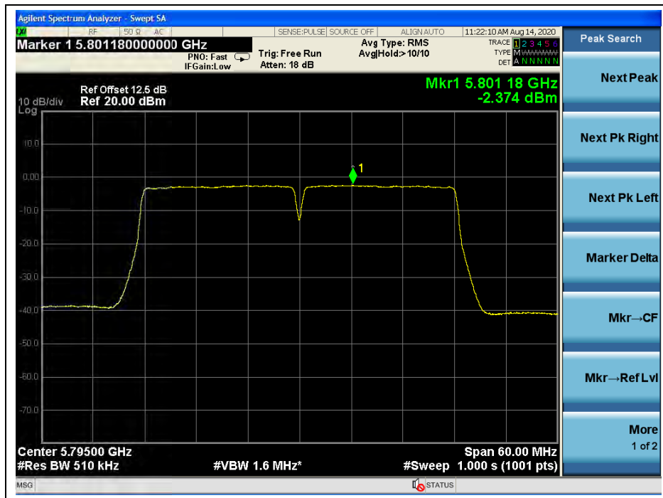
(Channel 159, 5795MHz, 802.11n (HT40), ANT R)
