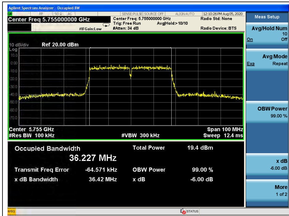
(Channel 151, 5755MHz, 802.11ac(VHT40))
