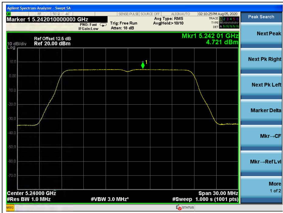
(Channel 48, 5240MHz, 802.11n (HT20), ANT L)
