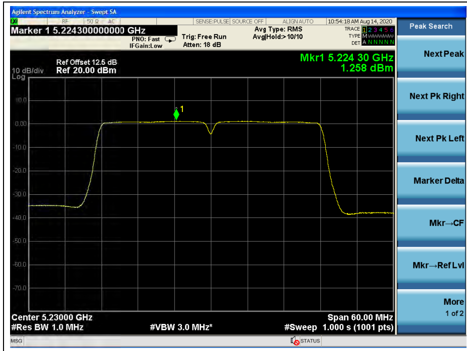
(Channel 46, 5230 MHz, 802.11ac (VHT40), ANT R)
