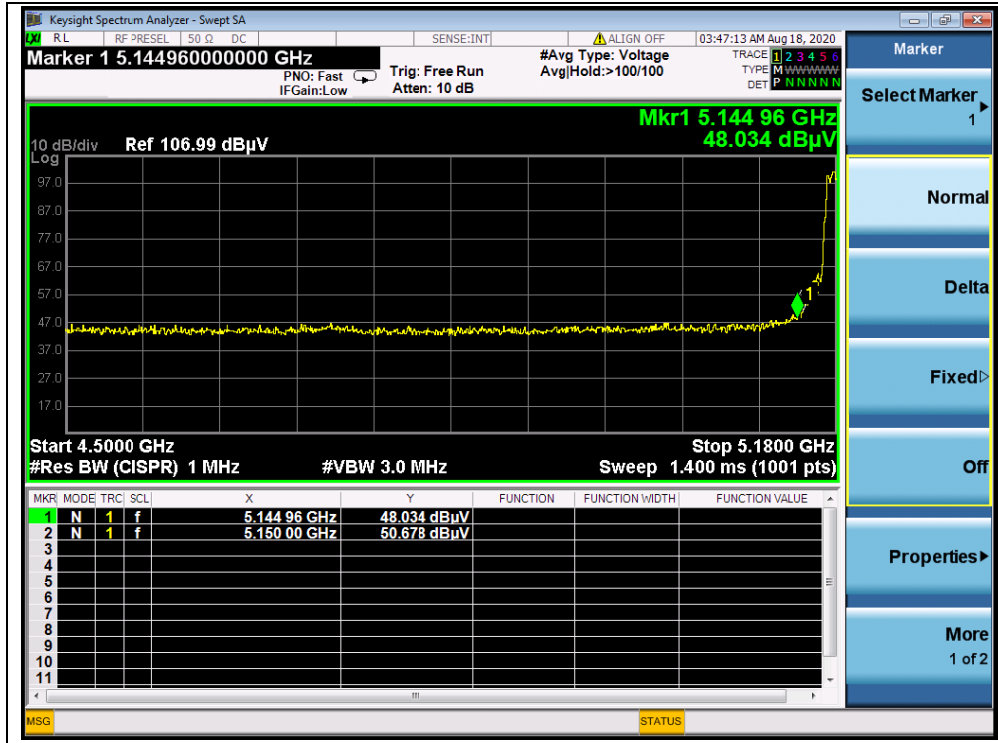
(PEAK,Channel 36,802.11a)
