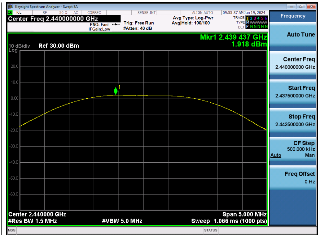
Test_Graph_LE2M_ANT1_2440_2Mbps_Peak Power
