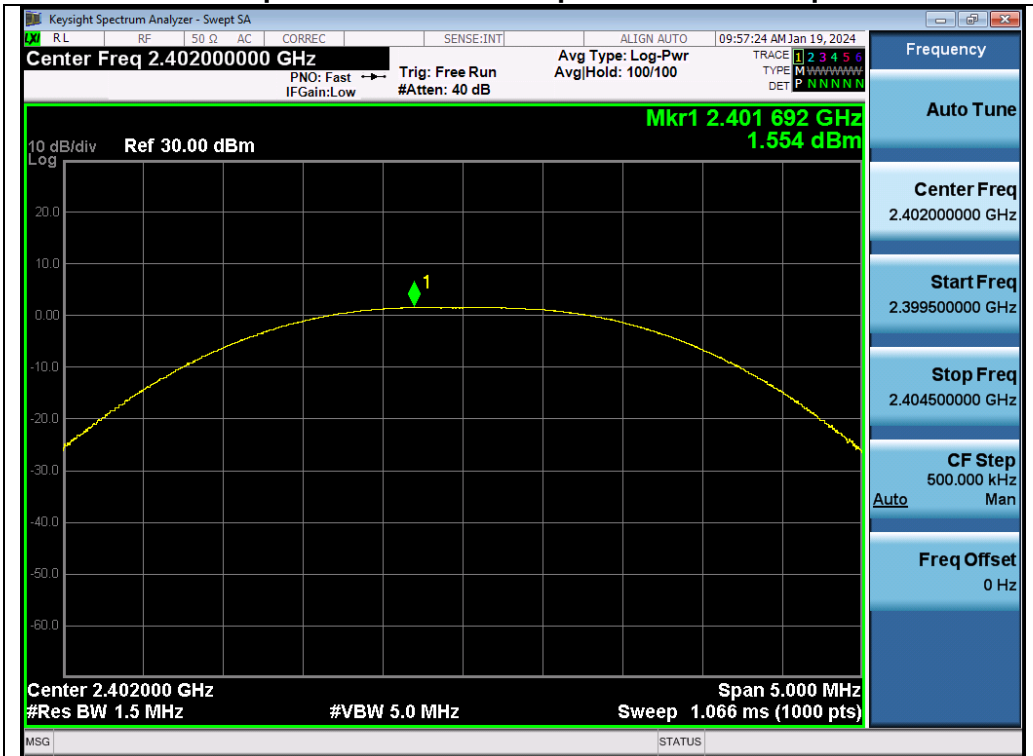
Test_Graph_BR_ANT1_2402_1Mbps_Peak Power
