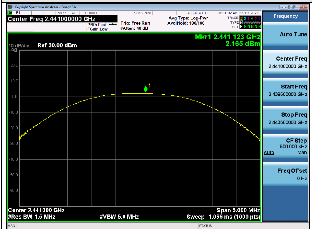
Test_Graph_BR_ANT1_2441_1Mbps_Peak Power
