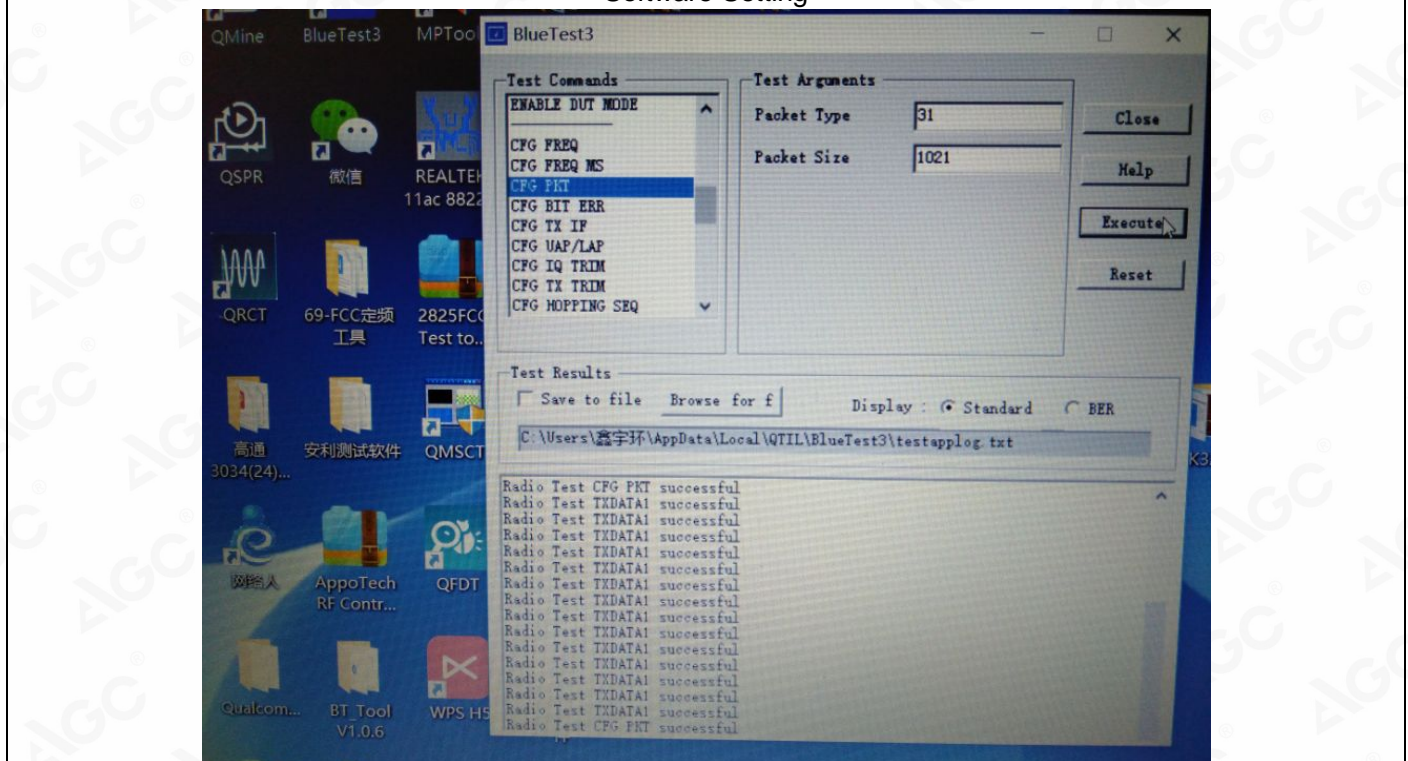
Software Setting
