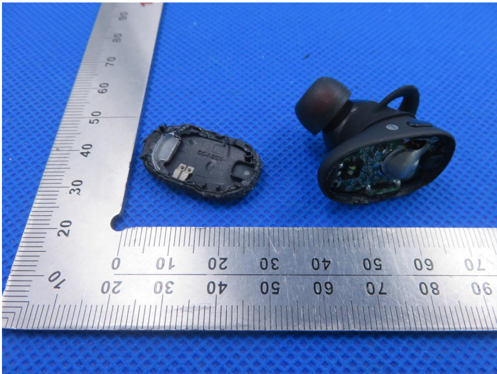
A3913 OPEN VIEW OF EUT
