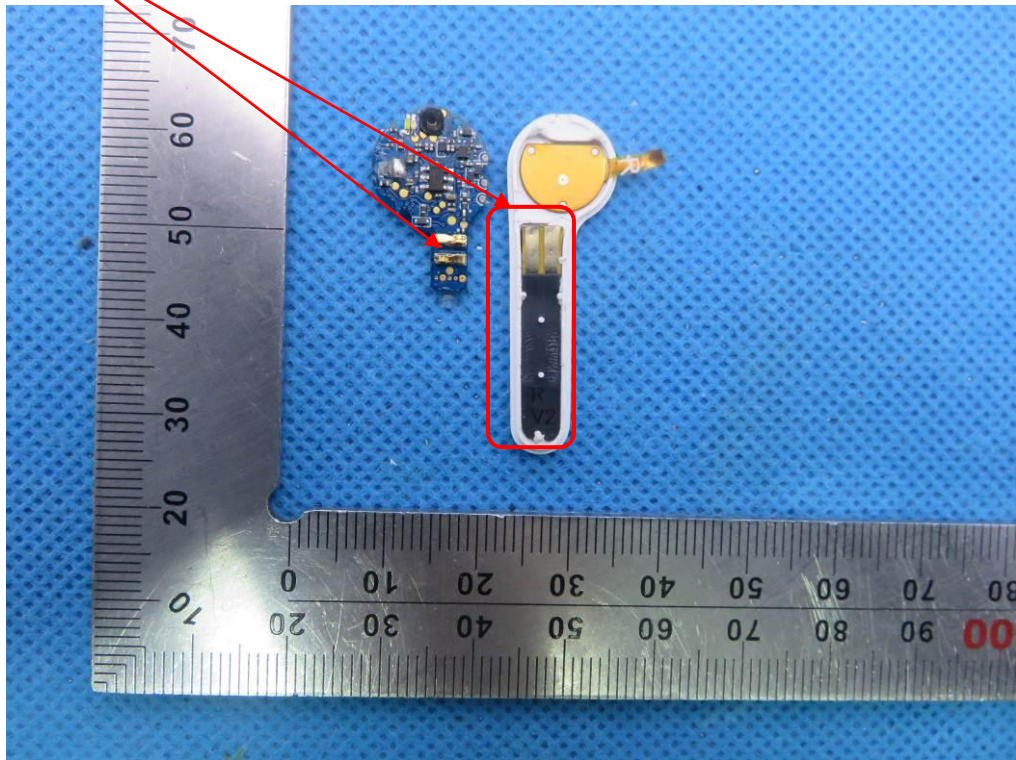
ANTENNA(right)
