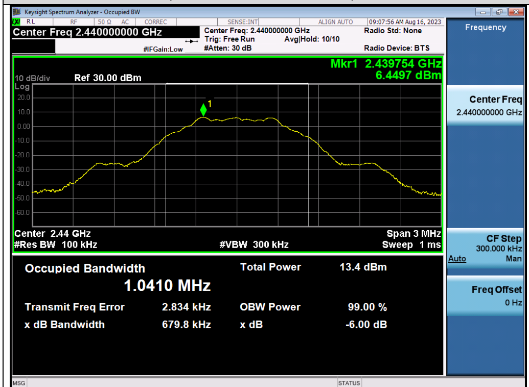
Test_Graph_LE1M_ANT1_2440_1Mbps_DTBSW
