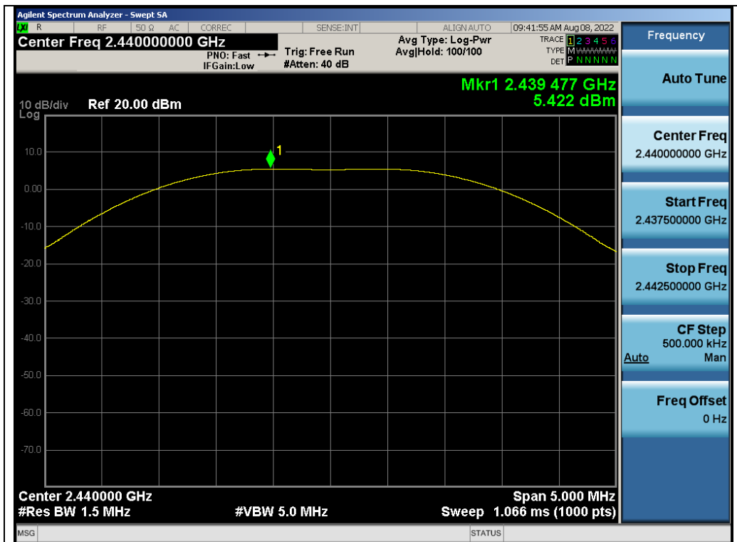
Test_Graph_GFSK_ANT1_2440_2Mbps_Peak Power
