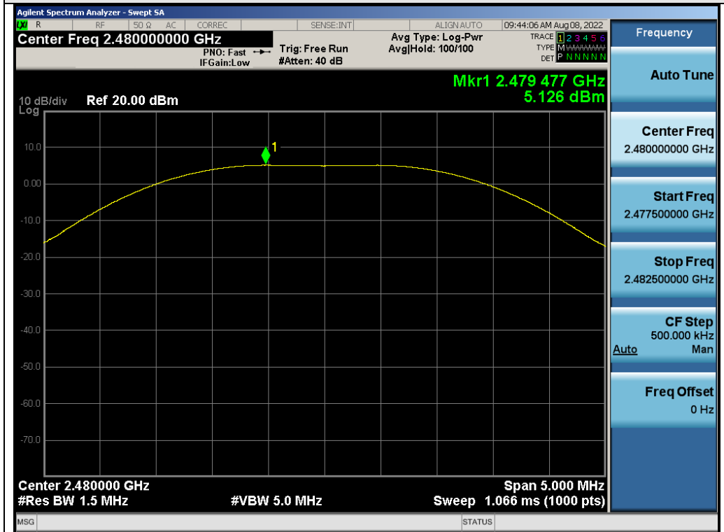
Test_Graph_GFSK_ANT1_2480_2Mbps_Peak Power
