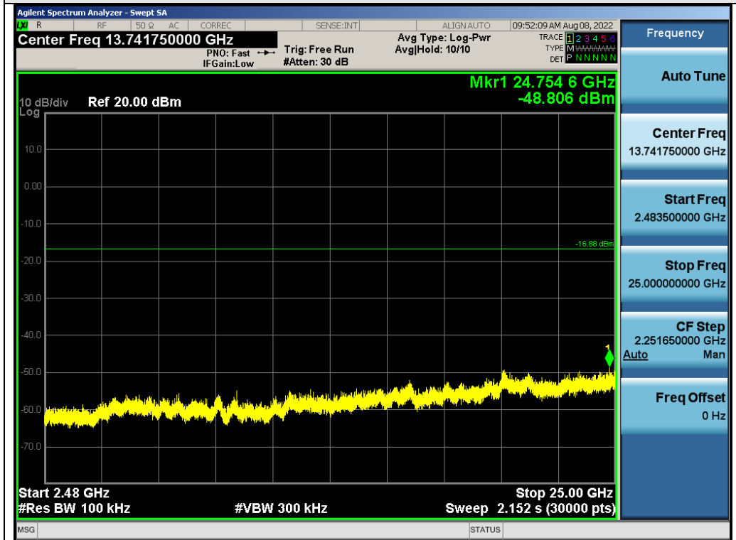
Test_Graph_GFSK_ANT1_2440_2Mbps_Higher Band Emissions
