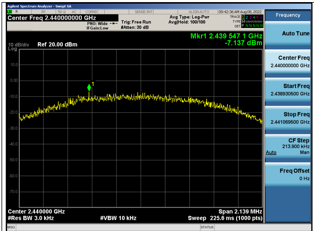
Test_Graph_GFSK_ANT1_2440_2Mbps_PSD
