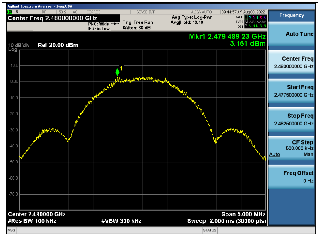
Test_Graph_GFSK_ANT1_2480_2Mbps_Reference Level
