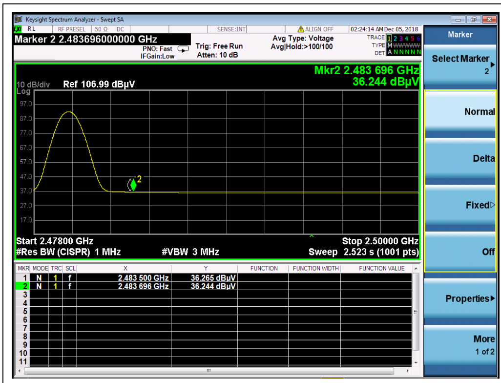
(Channel = 78, AVERAGE, GFSK)
