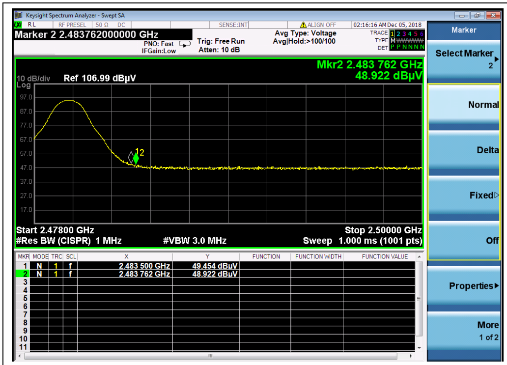
(Channel = 78, PEAK, 8-DPSK)
