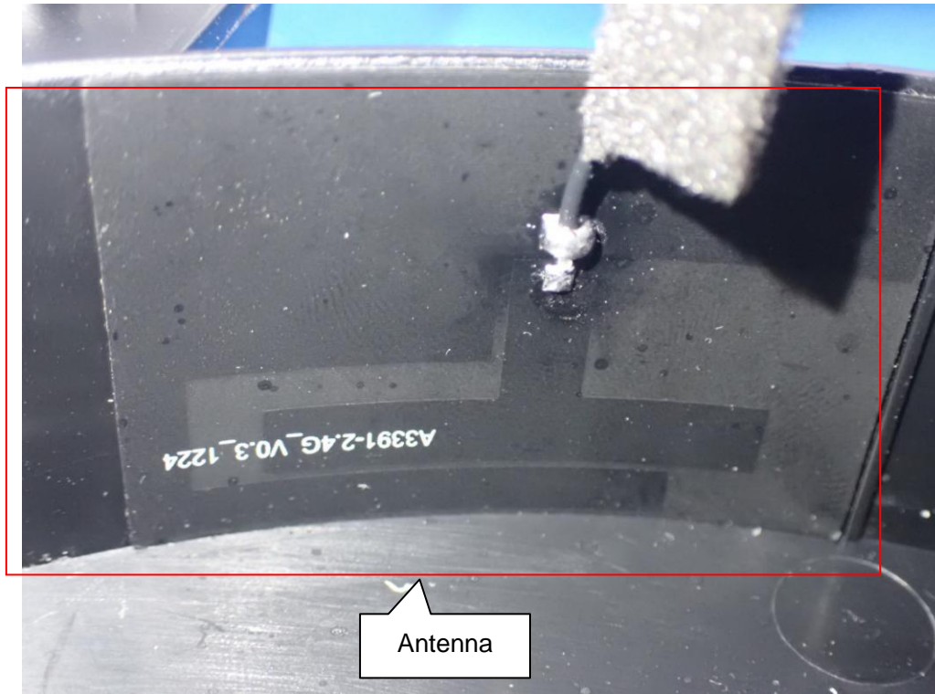
INTERNAL VIEW-14 OF EUT
