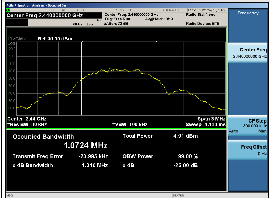
Test_Graph_2.4G_ANT1_2440_OBW
