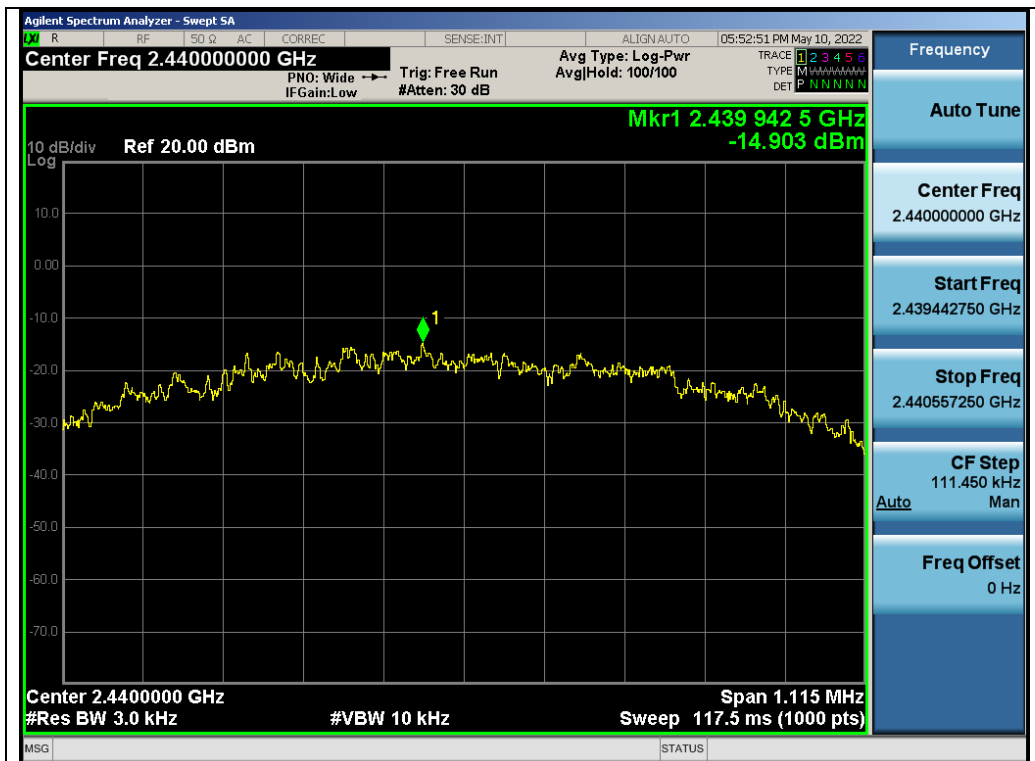
Test_Graph_2.4G_ANT1_2440_PSD
