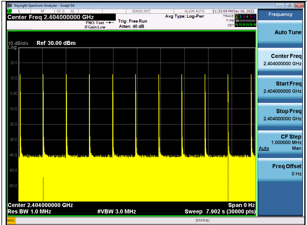
Test_Graph_2.4G_HOP_ANT2_NA_1Mbps_2404_Number of Burst
