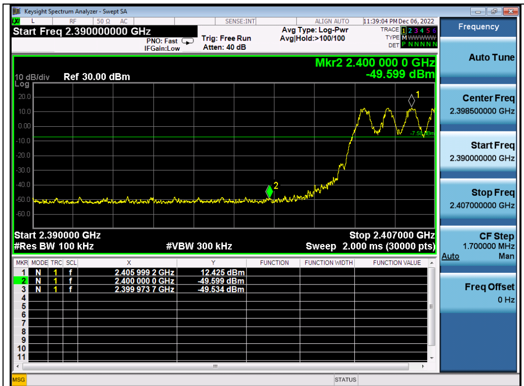
Test_Graph_2.4G_HOP_ANT2_NA_1Mbps_Lower Band Edge Emissions
