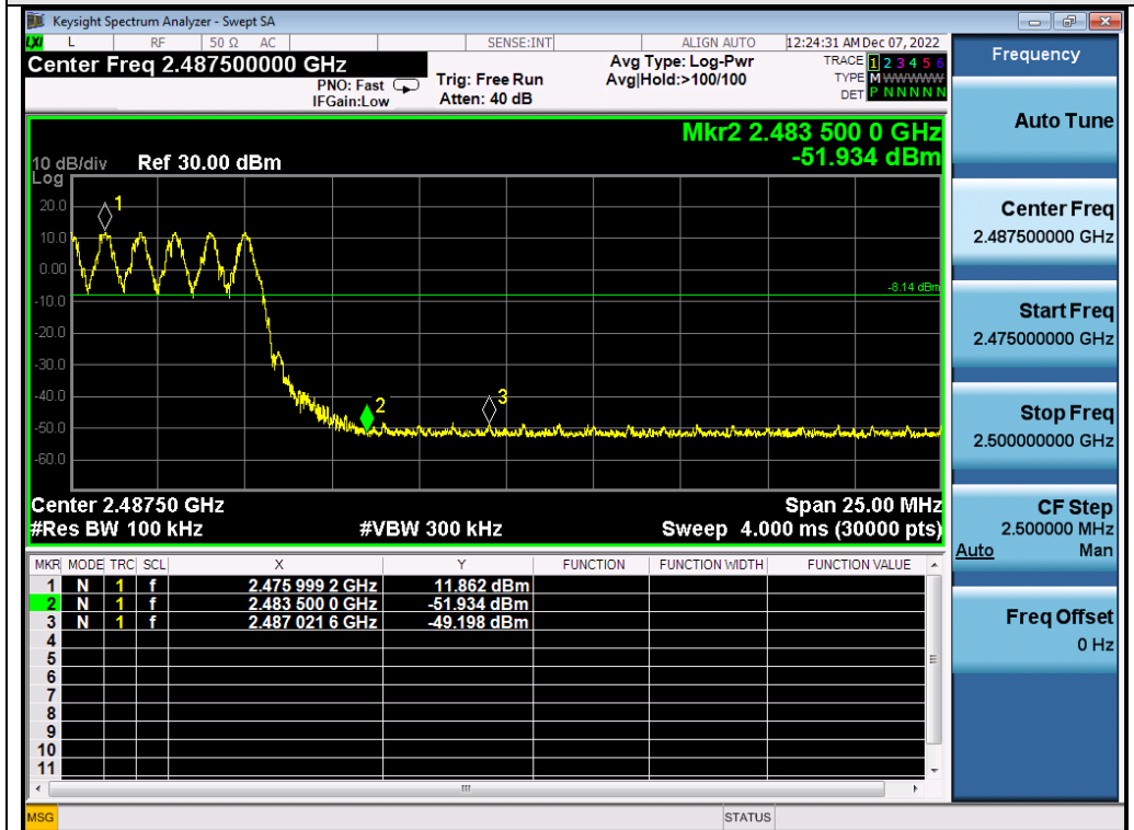
Test_Graph_2.4G_HOP_ANT2_NA_1Mbps_Higher Band Edge Emissions
