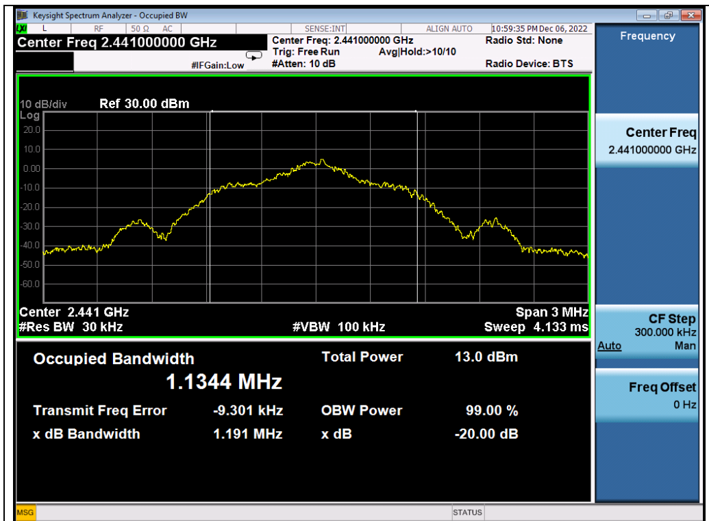
Test_Graph_2.4G_ANT2_2441_1Mbps_OBW
