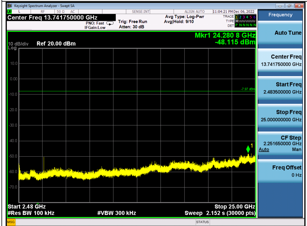
Test_Graph_2.4G_ANT2_2441_1Mbps_Higher Band Emissions
