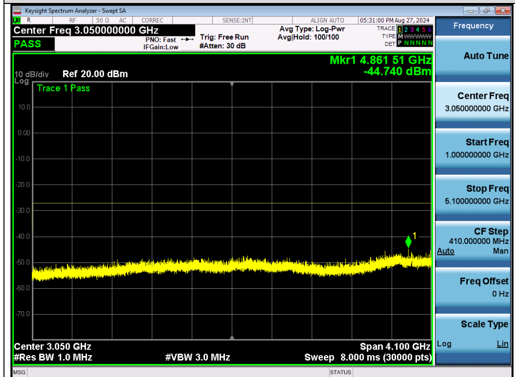
Test_Graph_802.11a_ANT1_5240_6Mbps_Frequency Band 2
