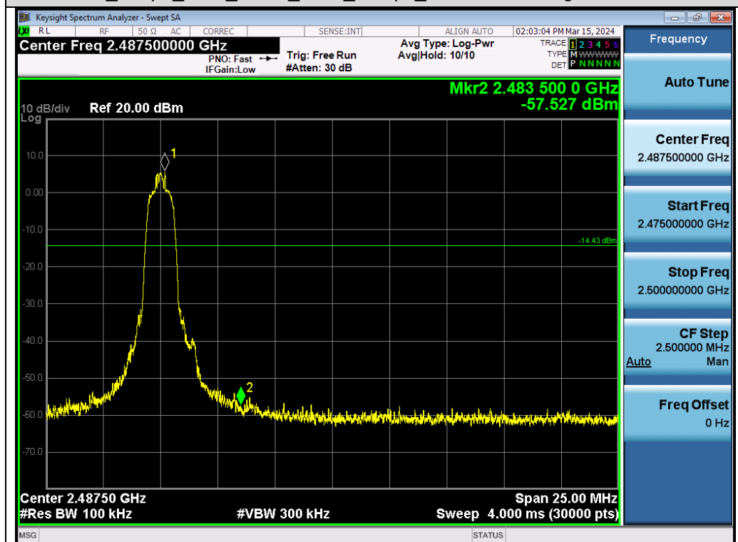
Test Graph EDR ANT1 2480 2Mbps Higher Band Edge Emissions
