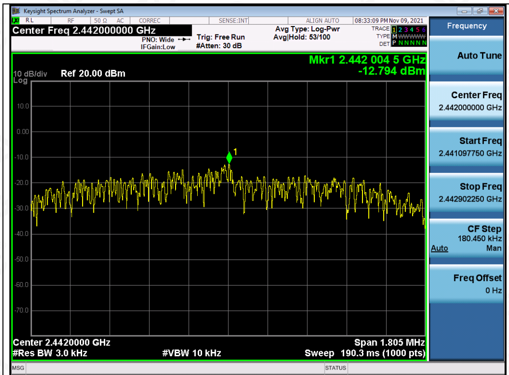
Test_Graph_LE2M_ANT1_2442_2Mbps_PSD
