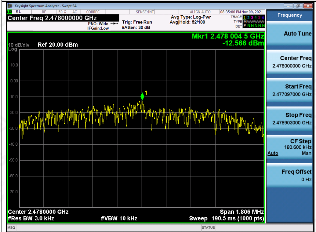
Test_Graph_LE2M_ANT1_2478_2Mbps_PSD
