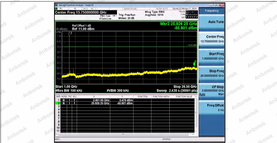
BLE_1M-Ant1-2402-1000~26500-PASS
