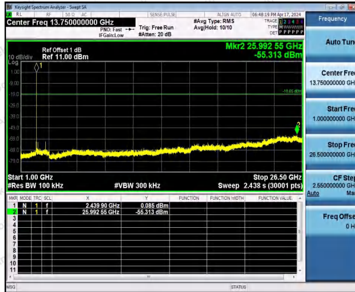
BLE_1M-Ant1-2440-1000~26500-PASS
