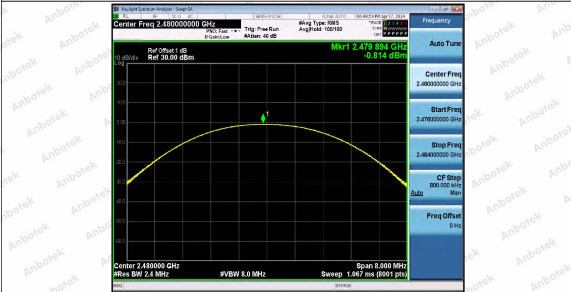
BLE_1M-Ant1-2480-PASS
