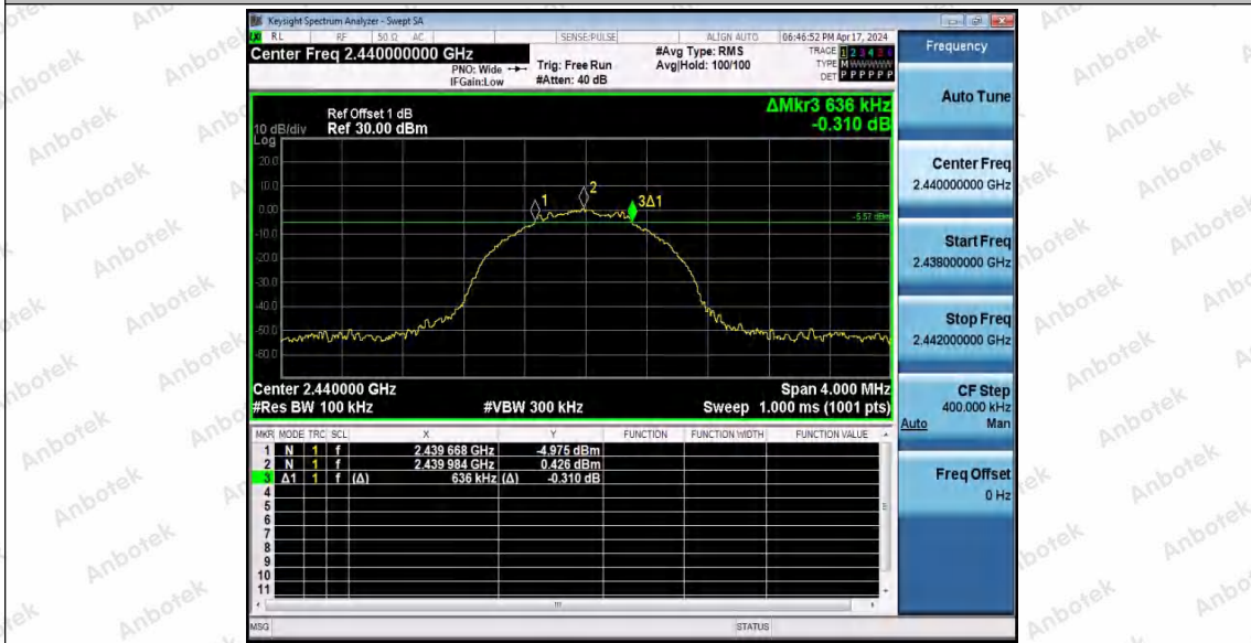
BLE_1M-Ant1-2440-PASS
