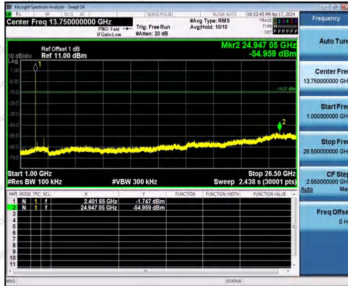
BLE_2M-Ant1-2402-1000~26500-PASS
