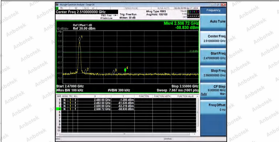
BLE_1M-Ant1-2480-PASS
