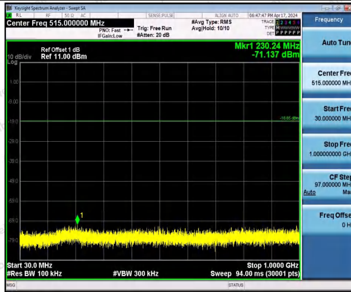
BLE_1M-Ant1-2440-30~1000-PASS
