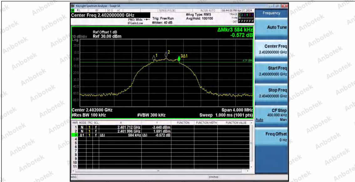
BLE_1M-Ant1-2402-PASS
