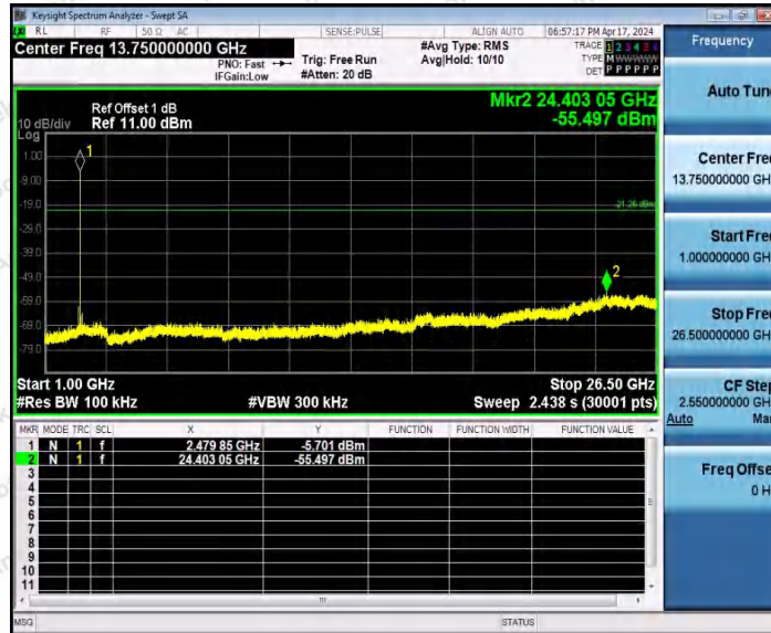
BLE_2M-Ant1-2480-1000~26500-PASS
