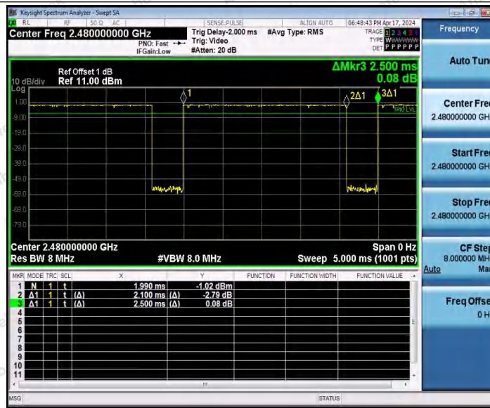
NTNV-BLE_1M-Ant1-2480
