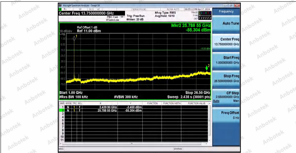
BLE_2M-Ant1-2440-1000~26500-PASS
