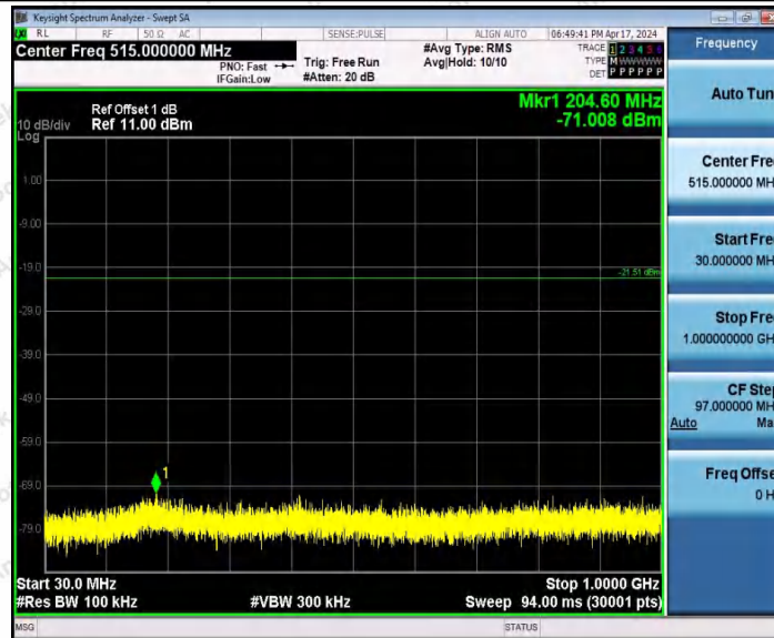
BLE_1M-Ant1-2480-30~1000-PASS
