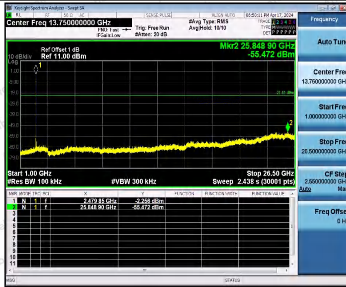
BLE_1M-Ant1-2480-1000~26500-PASS
