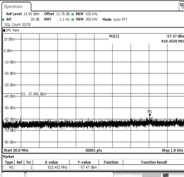
11N40SISO-Ant1-2437-30~1000-PASS
