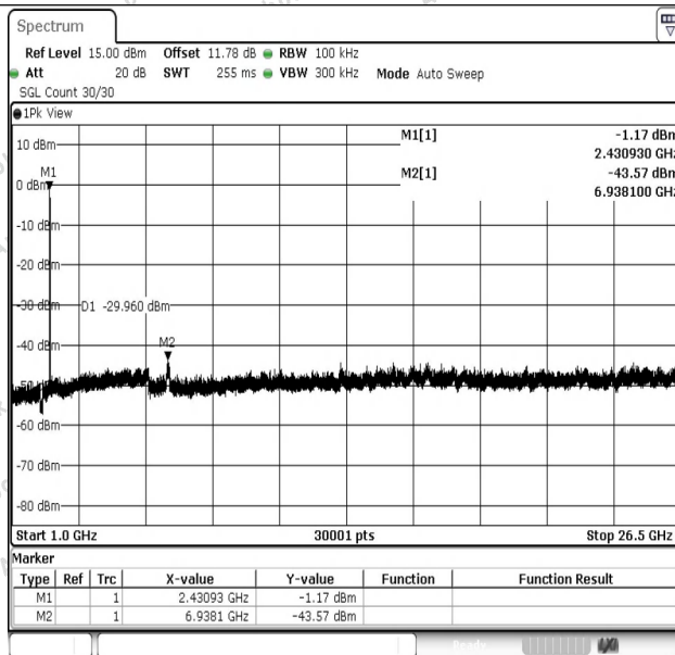
11G-Ant1-2437-1000~26500-PASS
