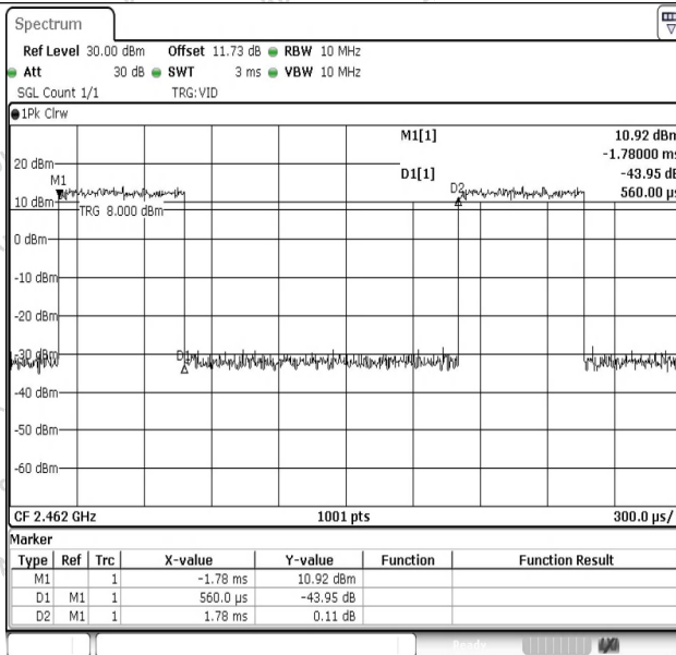
NTNV-11N20SISO-Ant1-2462
