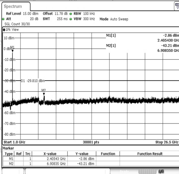
11N20SISO-Ant1-2412-1000~26500-PASS
