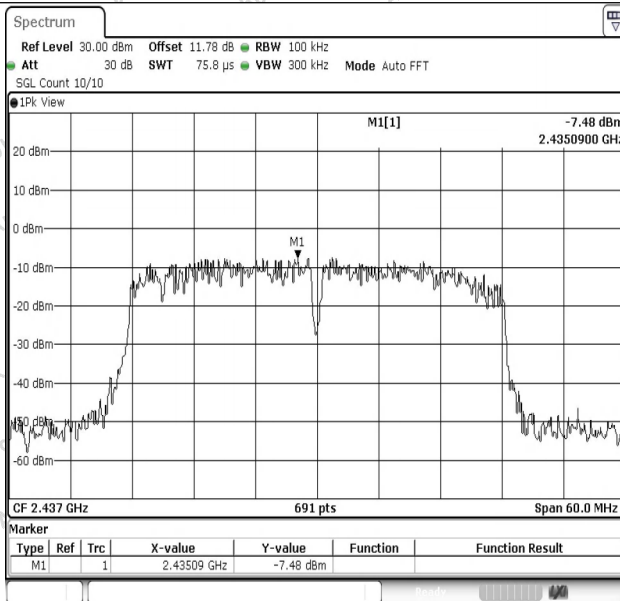
11N40SISO-Ant1-2437-0~Reference-PASS
