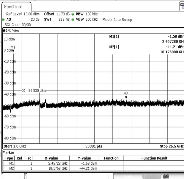
11N20SISO-Ant1-2462-1000~26500-PASS
