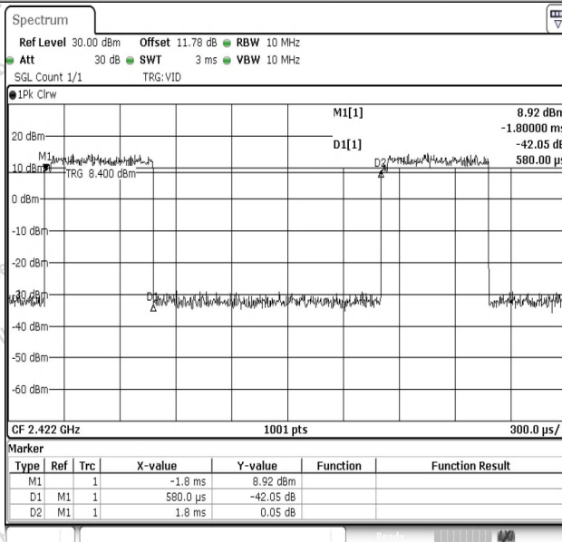
NTNV-11N40SISO-Ant1-2422
