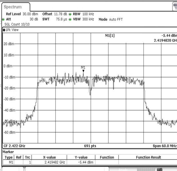
11N40SISO-Ant1-2422-0~Reference-PASS
