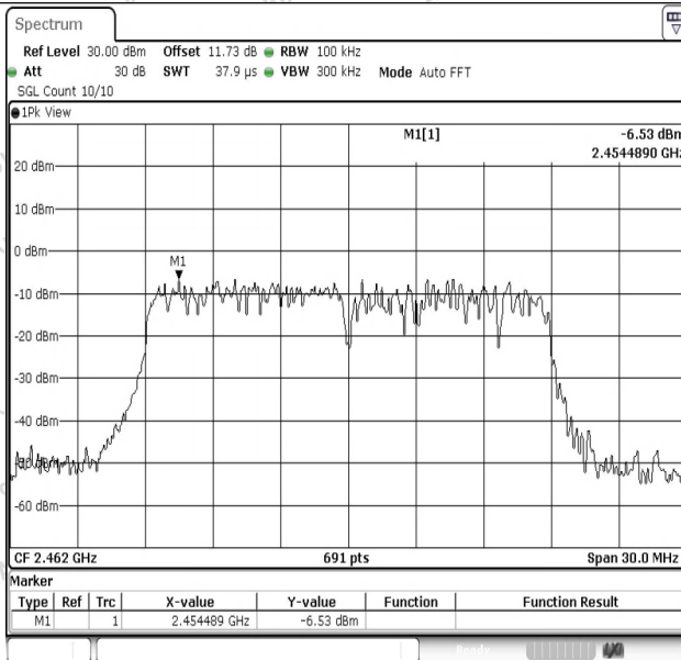
11N20SISO-Ant1-2462-0~Reference-PASS
