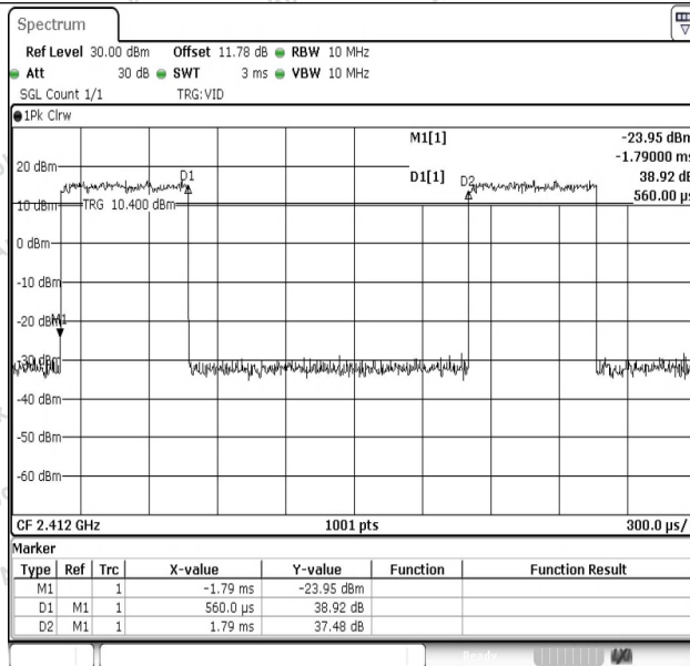
NTNV-11N20SISO-Ant1-2412
