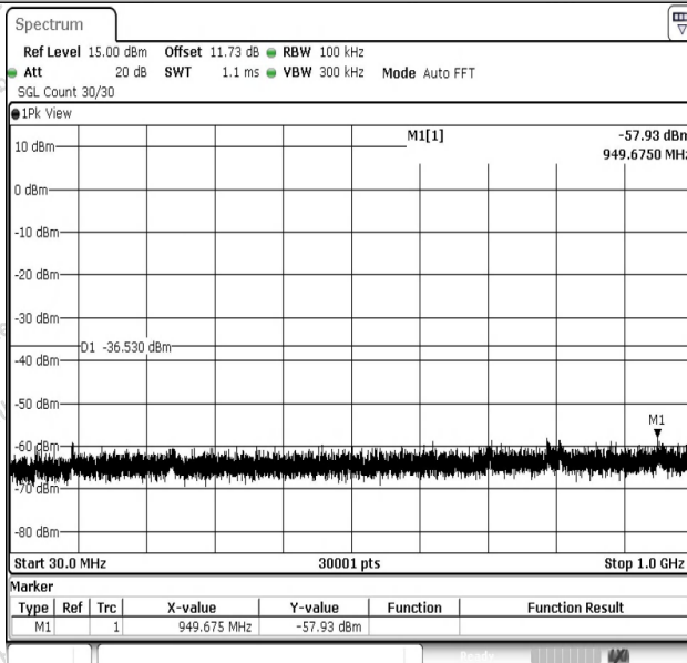
11N20SISO-Ant1-2462-30~1000-PASS
