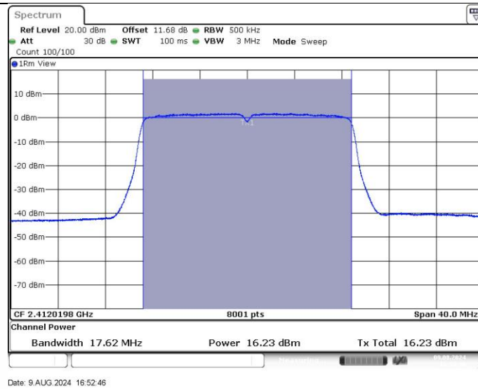
11N20SISO Ant1 2412
