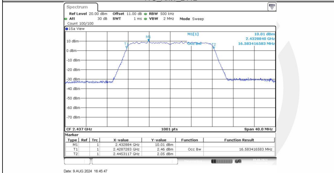
11G Ant1_2437
