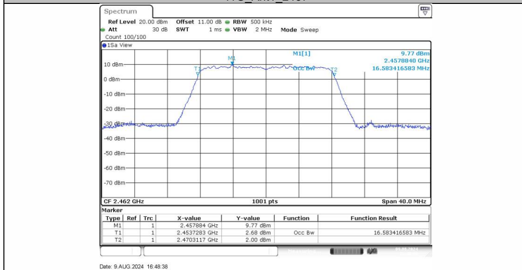
11G Ant1_2462
