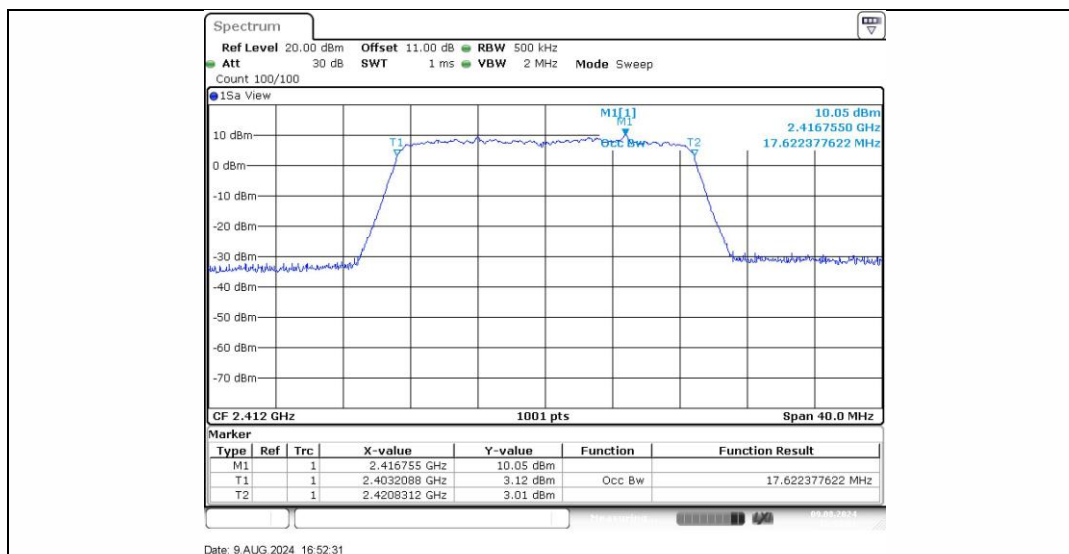
11N20SISO Ant1 2412
