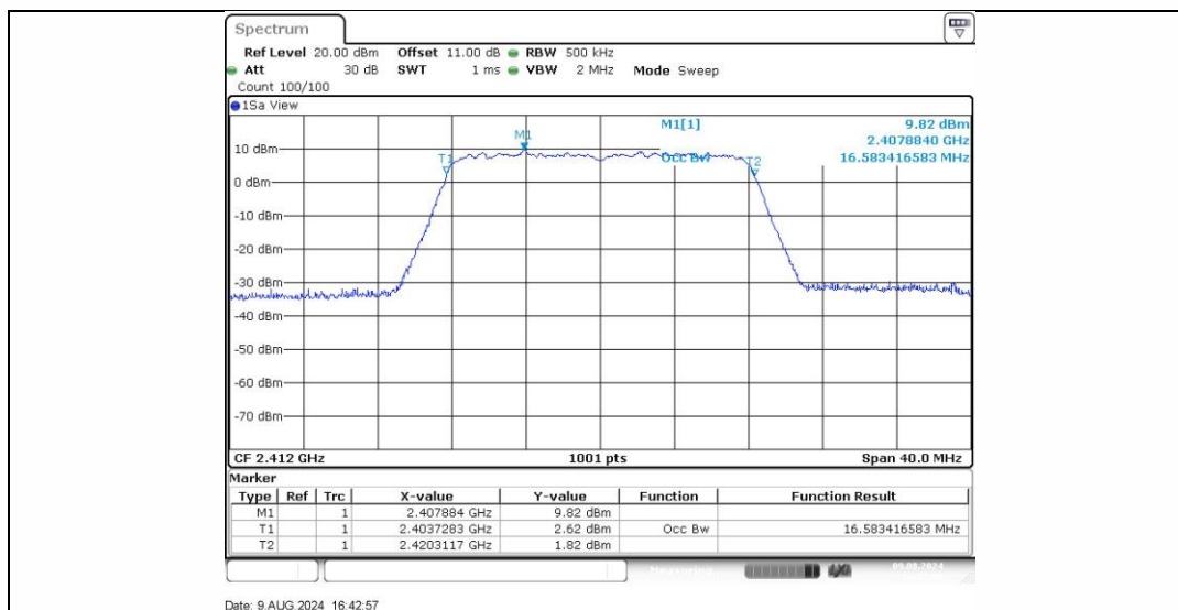
11G Ant1_2412
