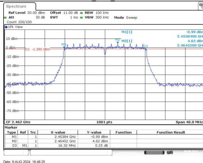
11G Ant1_2462
