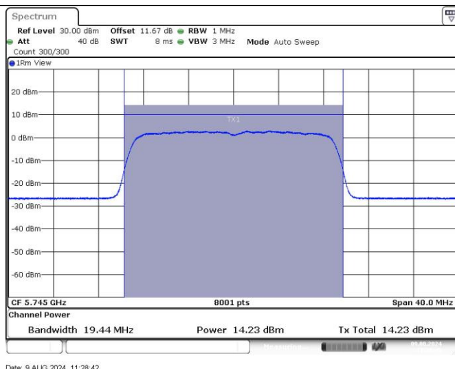
11AC20SISO_Ant1_5745
