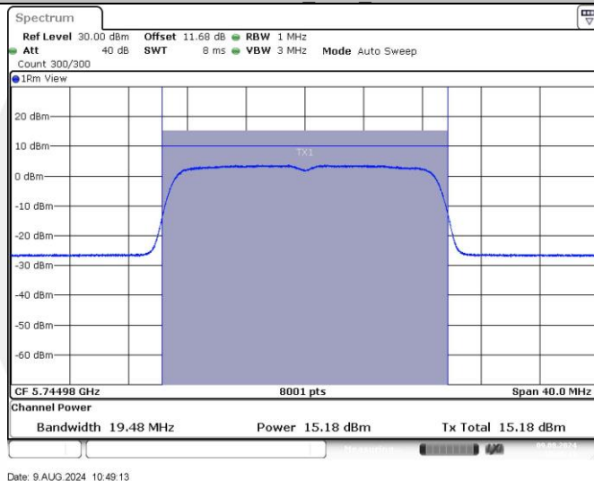
11N20SISO Ant1 5745
