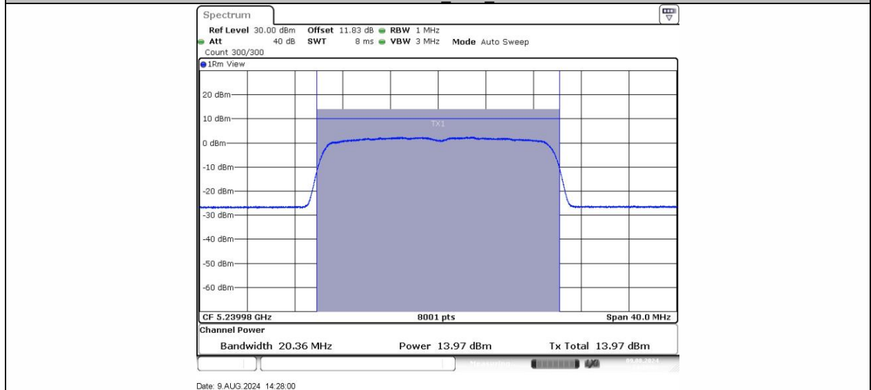
11AX20SISO Ant1 5240
