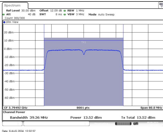
11AC40SISO Ant1 5795
