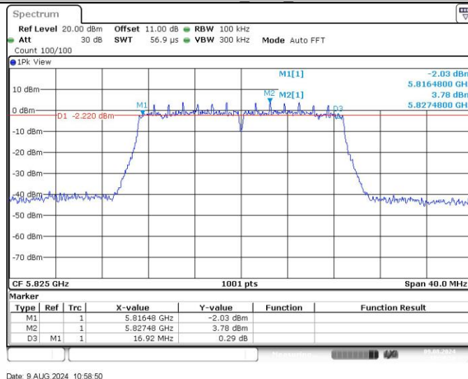
11N20SISO_Ant1_5825
