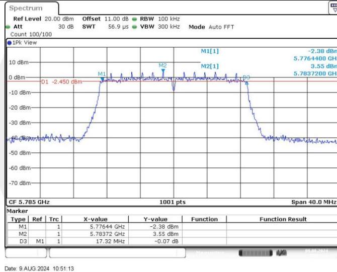
11N20SISO_Ant1_5785
