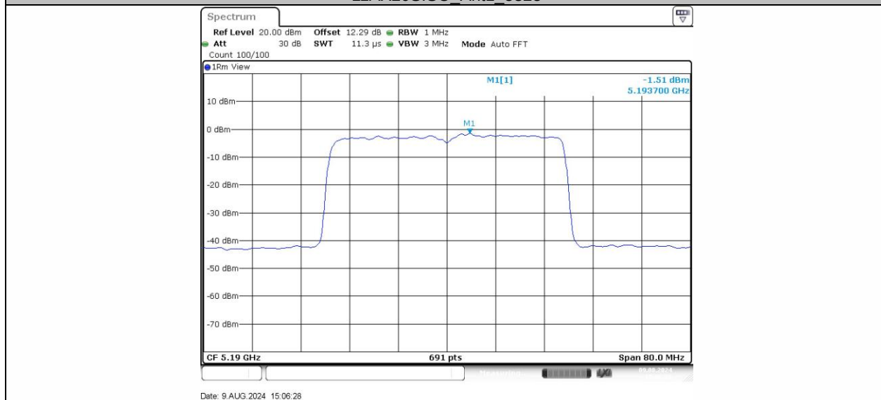
11AX40SISO Ant1 5190
