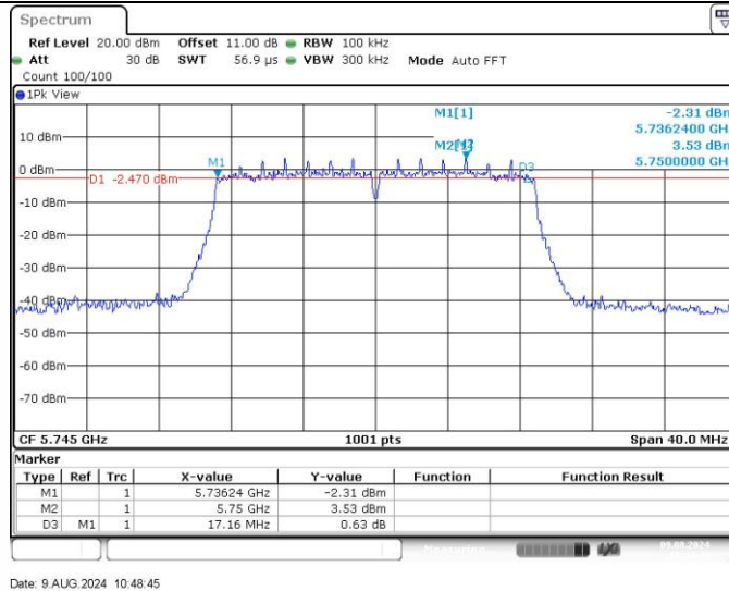
11N20SISO_Ant1_5745
