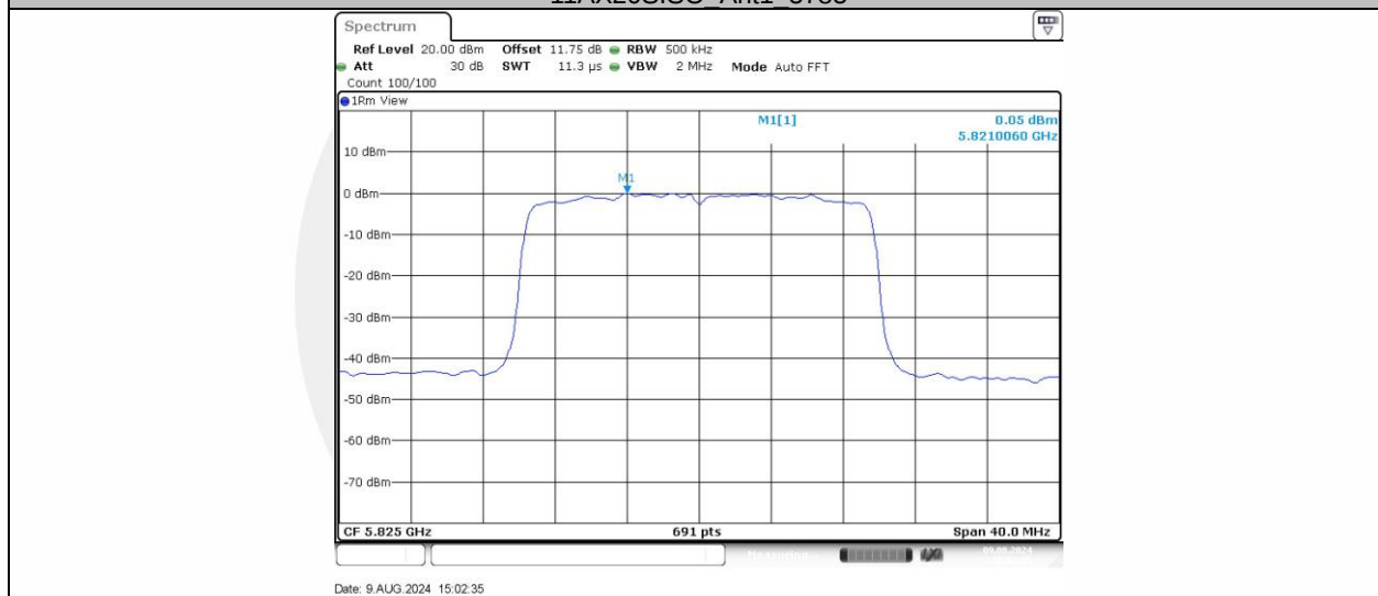
11AX20SISO Ant1 5825
