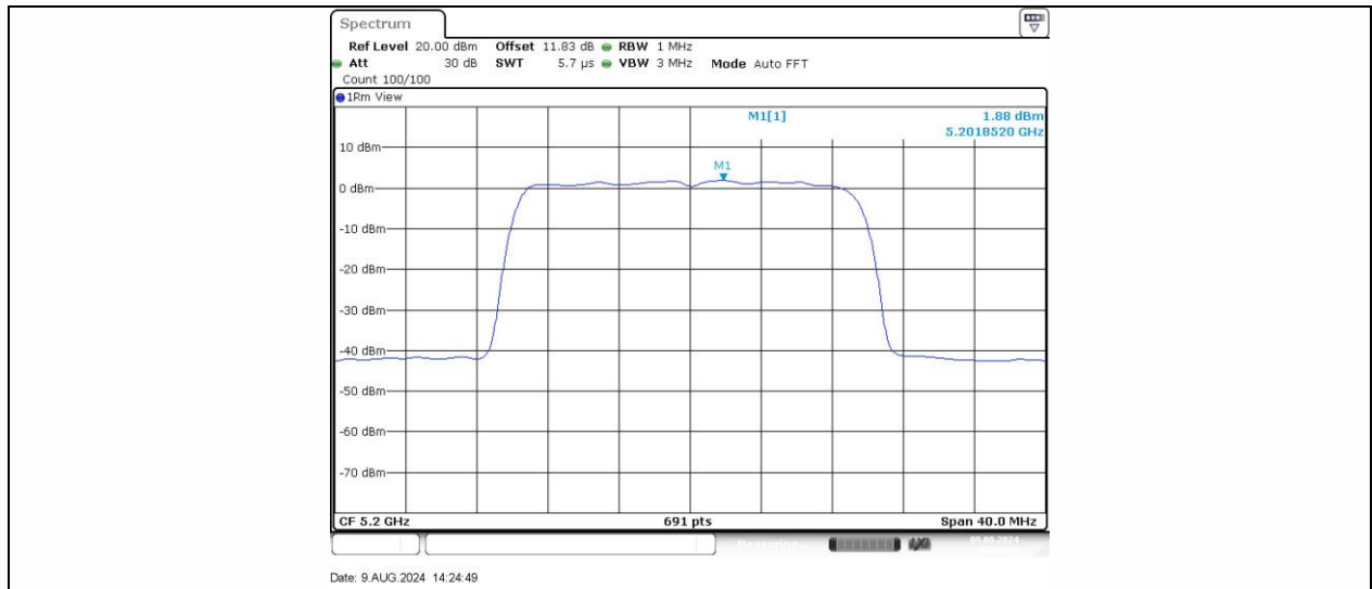
11AX20SISO Ant1 5200
