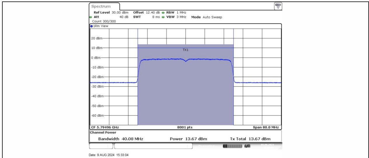
11AX40SISO Ant1 5795
