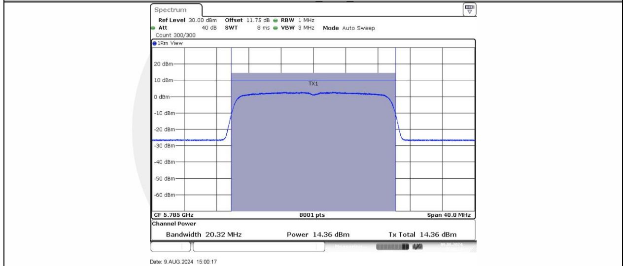
11AX20SISO Ant1 5785
