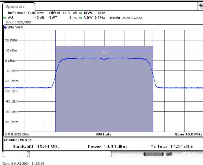
11AC20SISO_Ant1_5825
