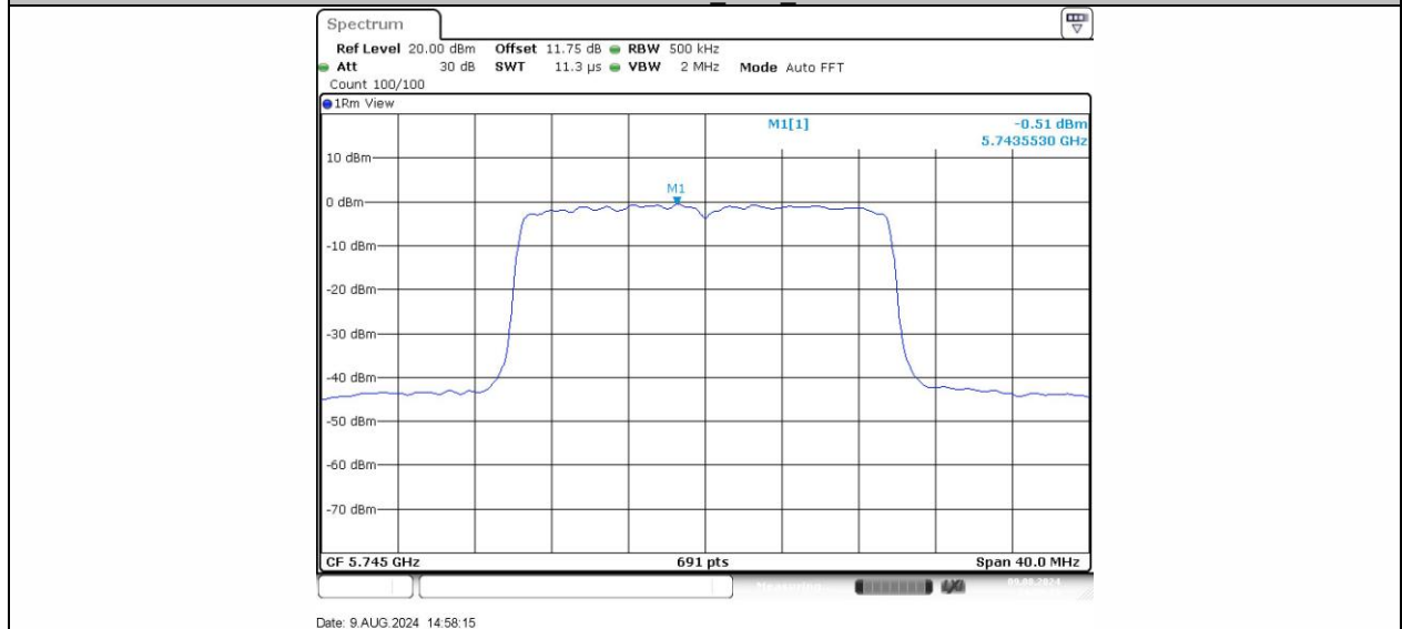
11AX20SISO Ant1 5745
