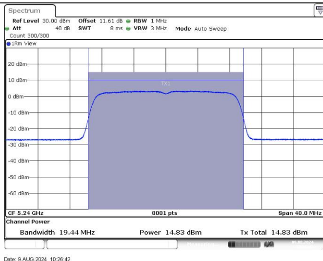
11N20SISO Ant1 5240
