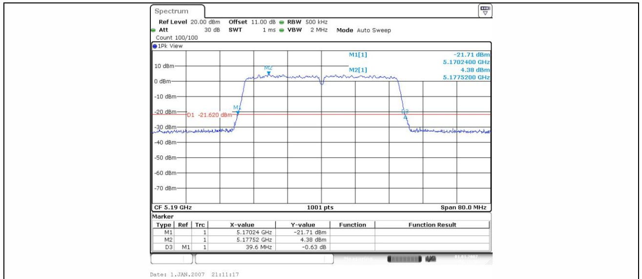
11N40SISO_Ant1_5190
