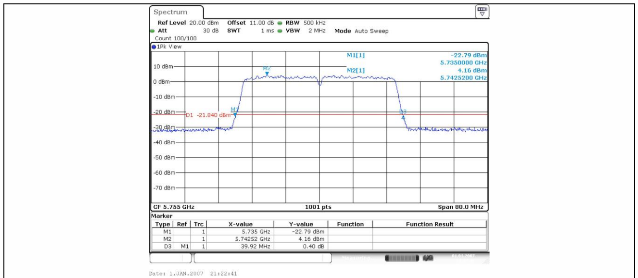
11N40SISO_Ant1_5755
