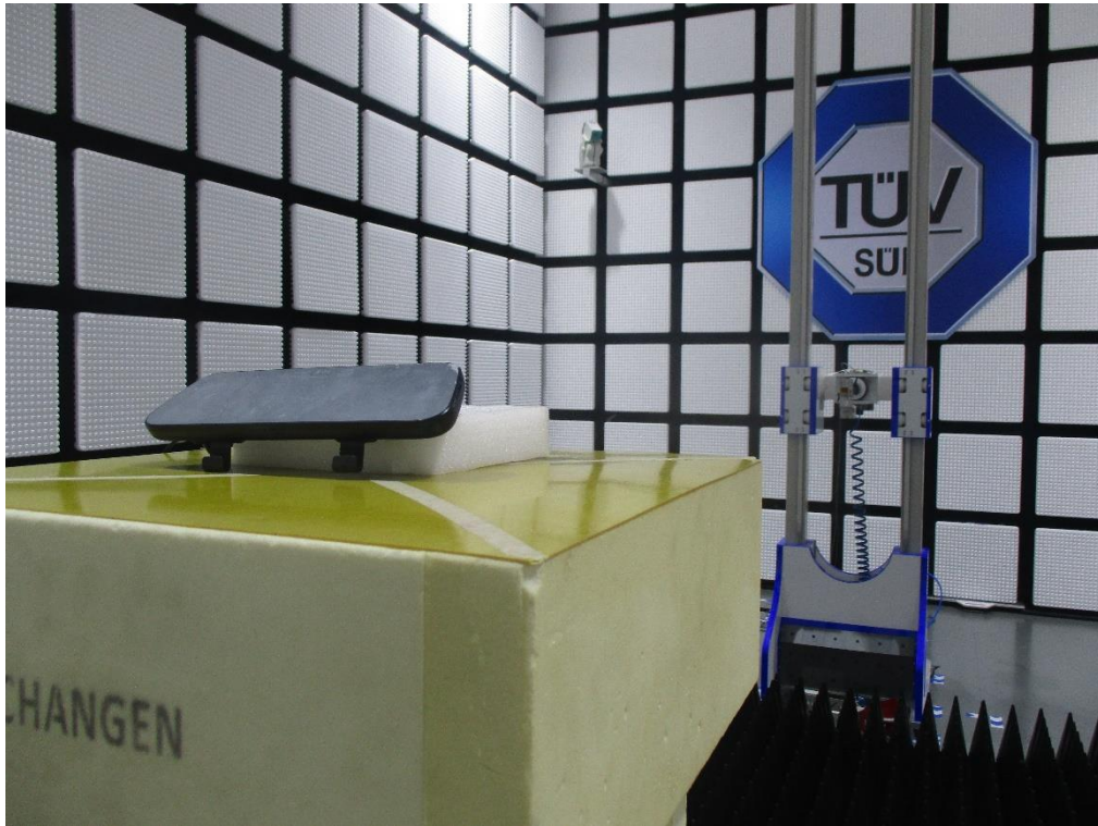
18GHz-40GHz RSE Setup
