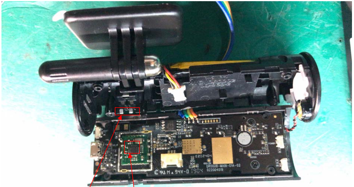
WIFI antenna WIFI module
