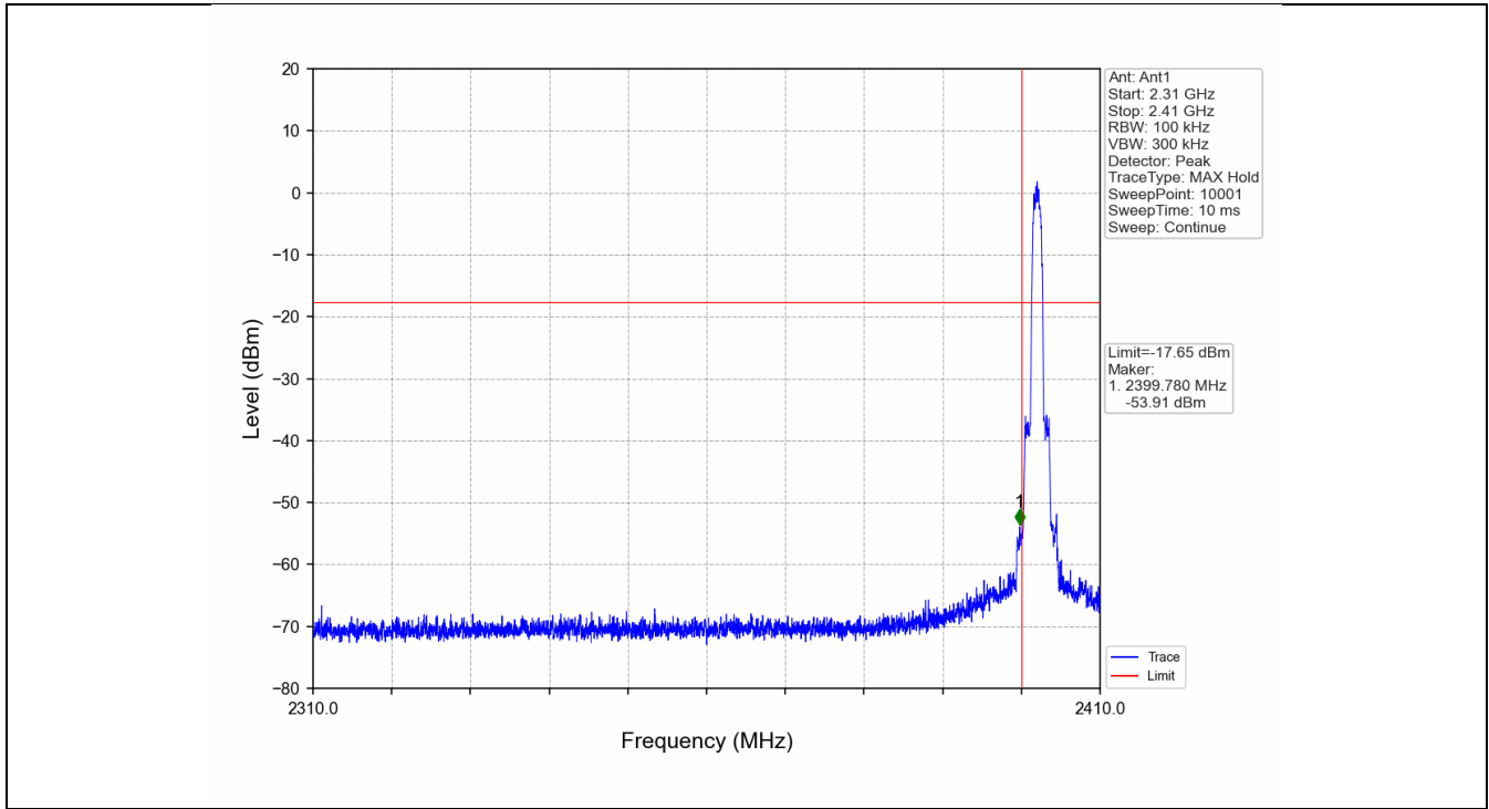
Pi/4DQPSK_2DH5_LCH_2402MHz_Ant1_NTNV
