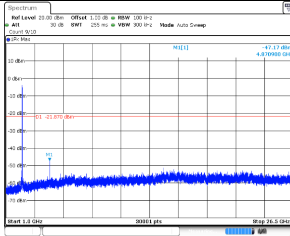
11G_Ant1_2437_1000~26500
