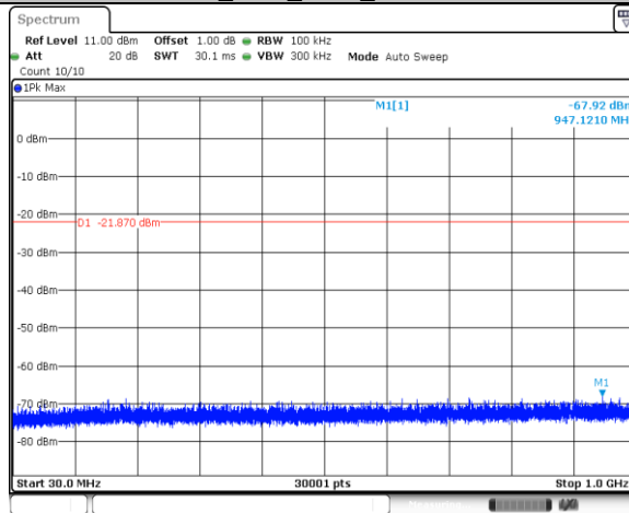
11G_Ant1_2437_30~1000
