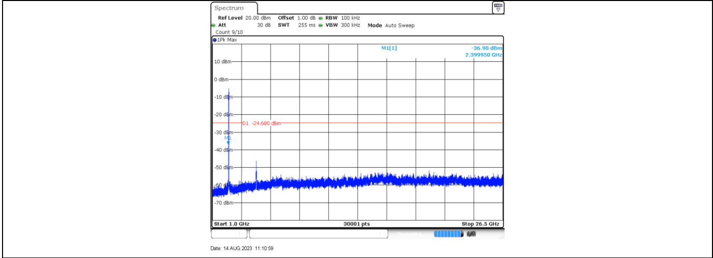
11N40SISO_Ant1_2437_0~Reference
