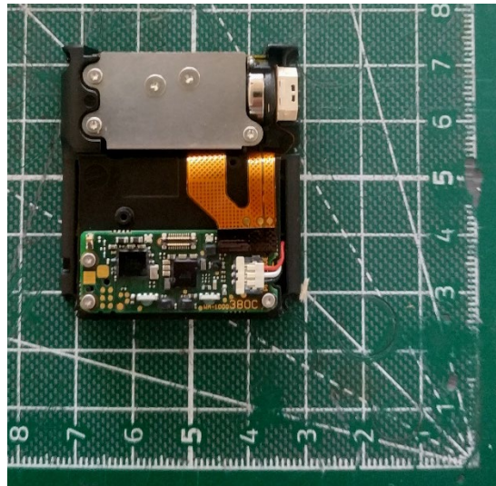
Figure 2: LEO internal top view
