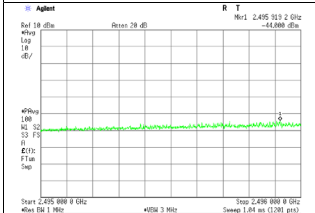
LTE Band 7 5MHz QPSK Low Channel RB1-0 2495MHz to 2496MHz Limit : -13dBm Pass
