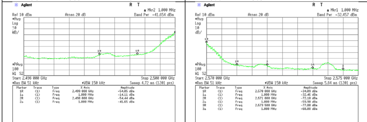
LTE Band 7 5MHz QPSK Low Channel RB1-0 2495MHz to 2496MHz Limit : -13dBm Pass
