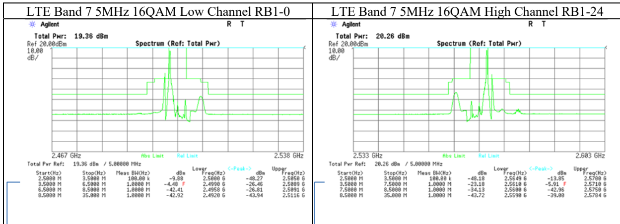
→ LTE Band 7 5MHz 16QAM Low Channel RB1-0 2496MHz to 2500MHz Limit : -10dBm Pass → LTE Band 7 5MHz 16QAM High Channel RB1-24 2570MHz to 2575MHz Limit : -10dBm Pass
