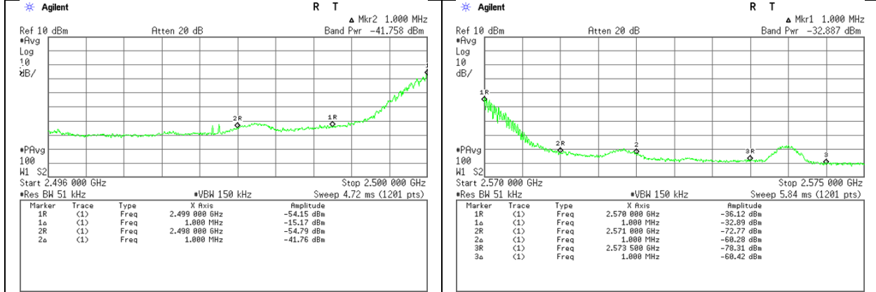
→ LTE Band 7 5MHz 16QAM Low Channel RB1-0 2496MHz to 2500MHz Limit : -10dBm Pass → LTE Band 7 5MHz 16QAM High Channel RB1-24 2570MHz to 2575MHz Limit : -10dBm Pass
