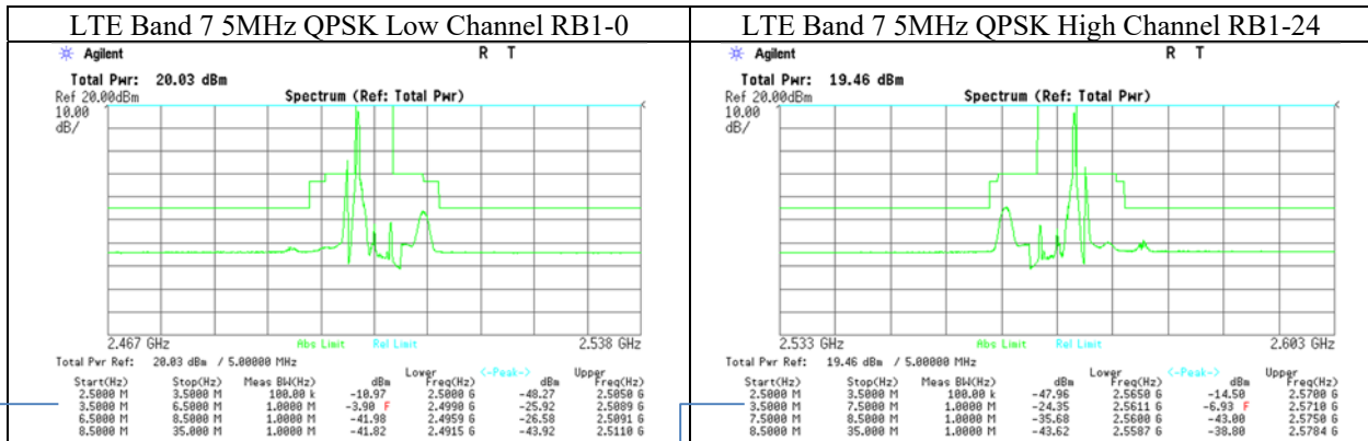
LTE Band 7 5MHz QPSK Low Channel RB1-0 2496MHz to 2500MHz Limit : -10dBm Pass
