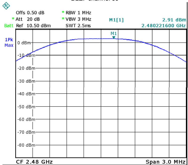
BLE: channel 39
