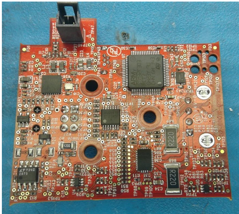
View of bottom side of main PCBA
