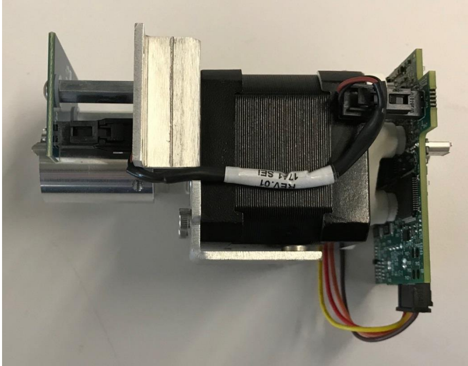
Side view of assembly containing, from left to right, the Antenna PCBA, stepper motor and main PCBA
