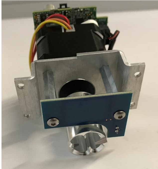
View of motor output shaft coupling and RFID antenna PCBA
