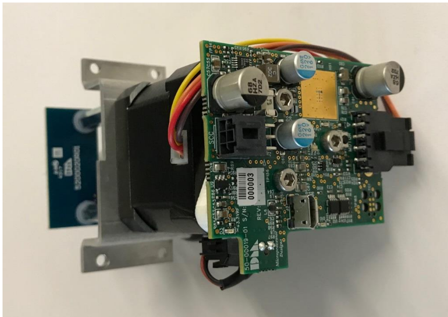
View of main controller PCBA mounted to back of motor
