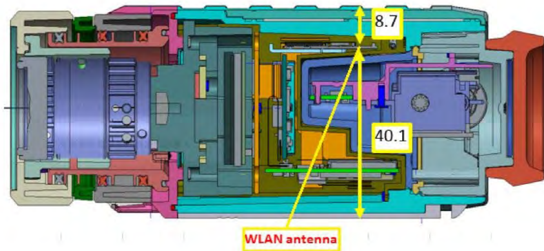
Fig.8 Antenna location
