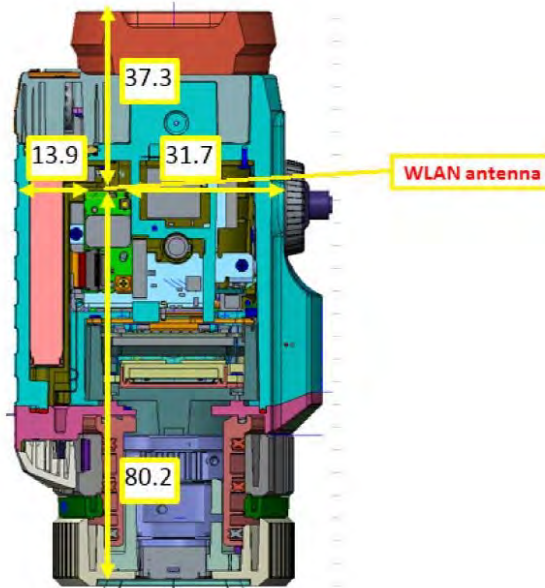
Fig.7 Antenna location
