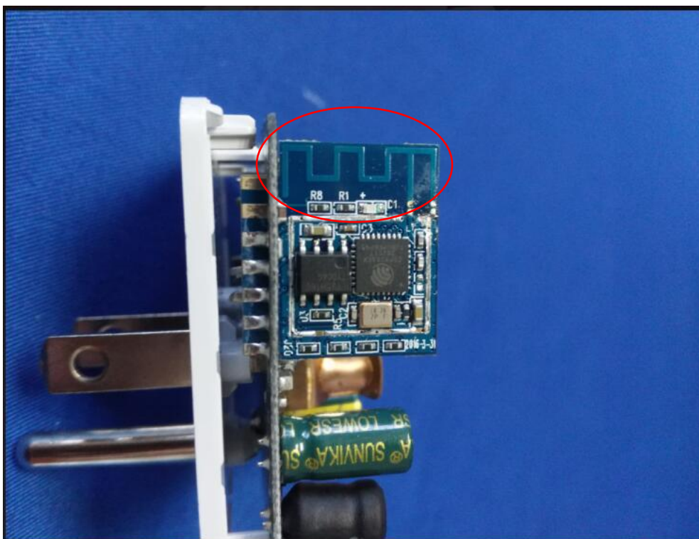
WIFI - Antenna View
